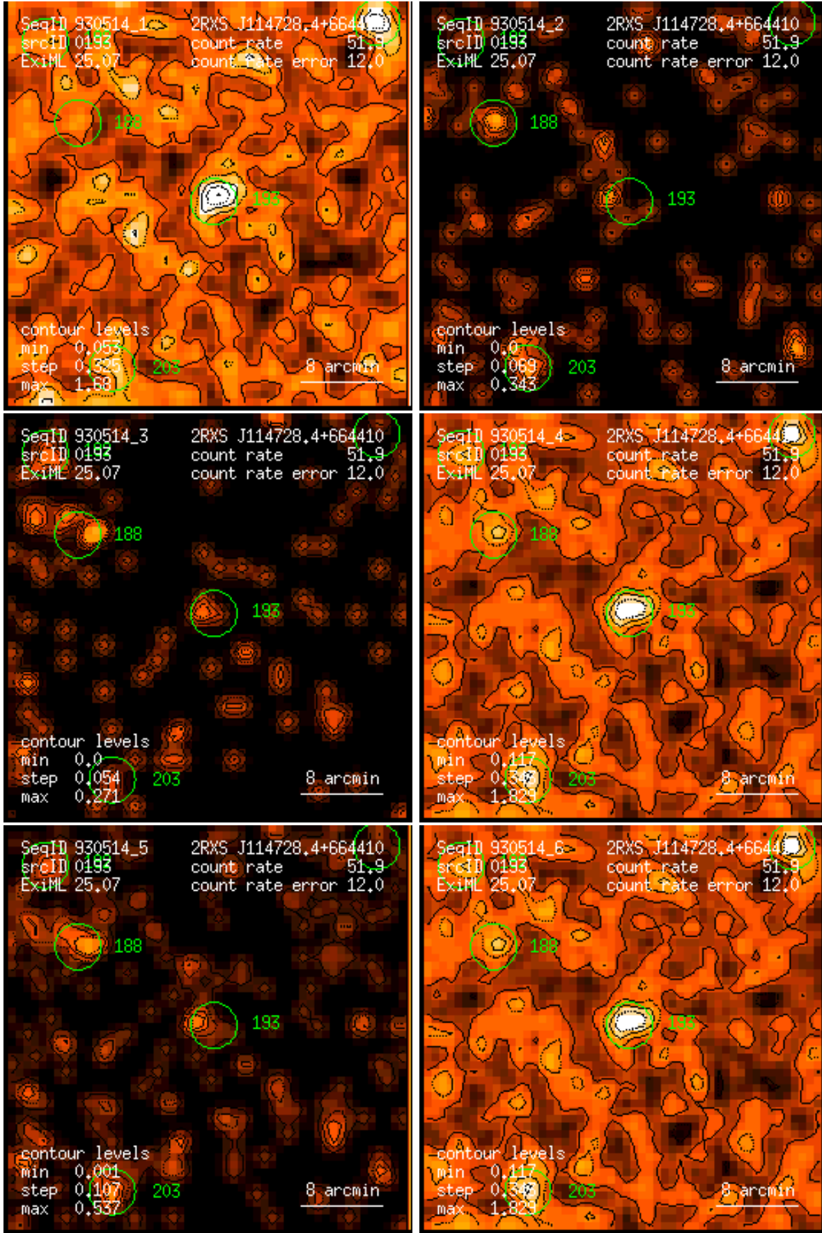
Figure 193: RASS 930514: detection 0193: band rate images, Gaussian filter: (1) PSPC channels 11 – 41, (2) 52 – 90, (3) 91 – 201, (4) 11 – 235, (5) 52 – 201, (6) 11 – 201. Broad band rates in counts/ks. Band rate contour levels in counts/ks/arcmin 2 .
