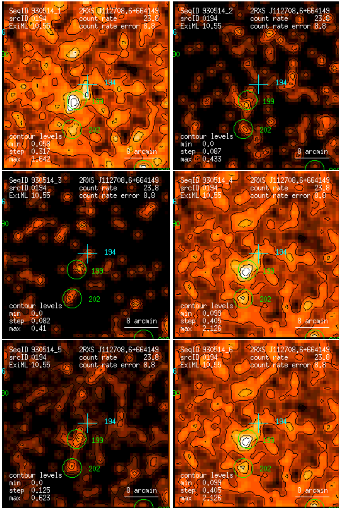
Figure 194: RASS 930514: detection 0194: band rate images, Gaussian filter: (1) PSPC channels 11 – 41, (2) 52 – 90, (3) 91 – 201, (4) 11 – 235, (5) 52 – 201, (6) 11 – 201. Broad band rates in counts/ks. Band rate contour levels in counts/ks/arcmin 2 .
