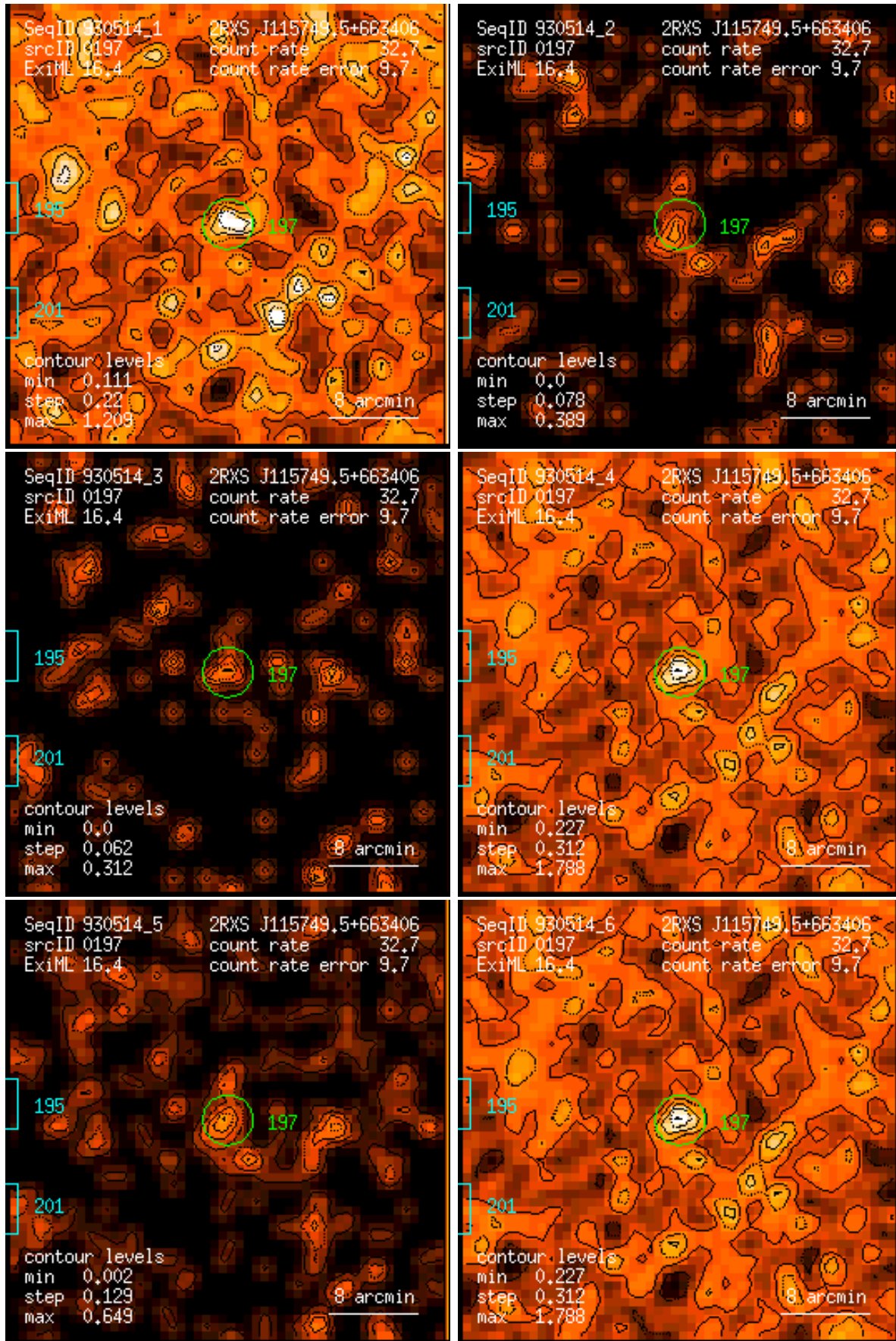
Figure 197: RASS 930514: detection 0197: band rate images, Gaussian filter: (1) PSPC channels 11 – 41, (2) 52 – 90, (3) 91 – 201, (4) 11 – 235, (5) 52 – 201, (6) 11 – 201. Broad band rates in counts/ks. Band rate contour levels in counts/ks/arcmin 2 .
