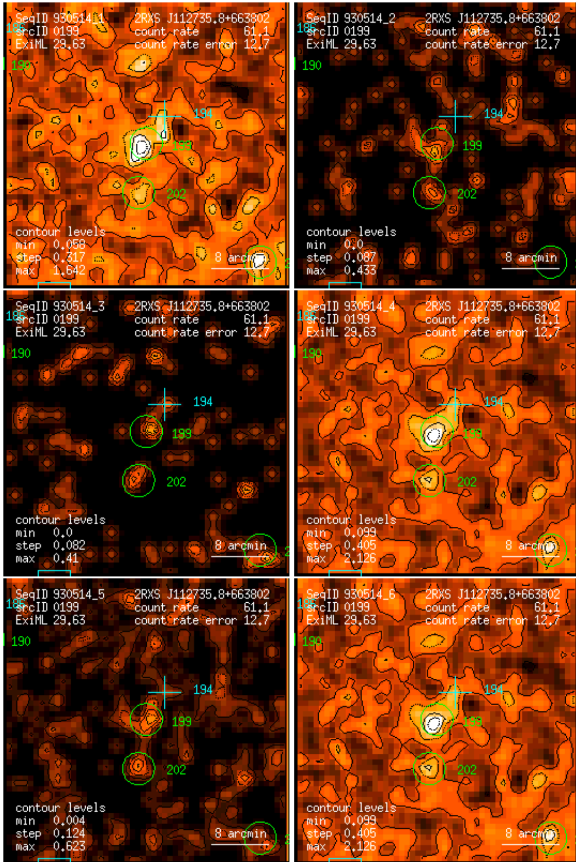
Figure 199: RASS 930514: detection 0199: band rate images, Gaussian filter: (1) PSPC channels 11 – 41, (2) 52 – 90, (3) 91 – 201, (4) 11 – 235, (5) 52 – 201, (6) 11 – 201. Broad band rates in counts/ks. Band rate contour levels in counts/ks/arcmin 2 .
