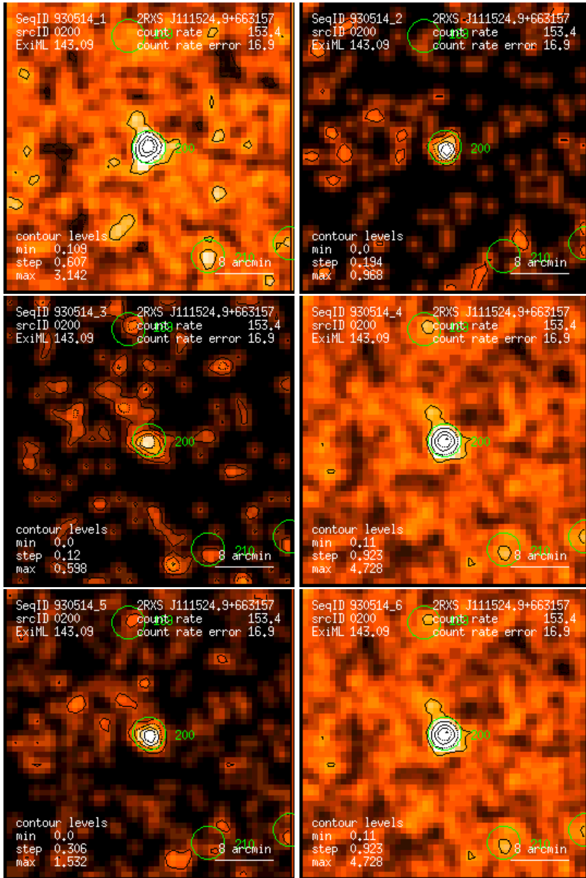
Figure 200: RASS 930514: detection 0200: band rate images, Gaussian filter: (1) PSPC channels 11 – 41, (2) 52 – 90, (3) 91 – 201, (4) 11 – 235, (5) 52 – 201, (6) 11 – 201. Broad band rates in counts/ks. Band rate contour levels in counts/ks/arcmin 2 .
