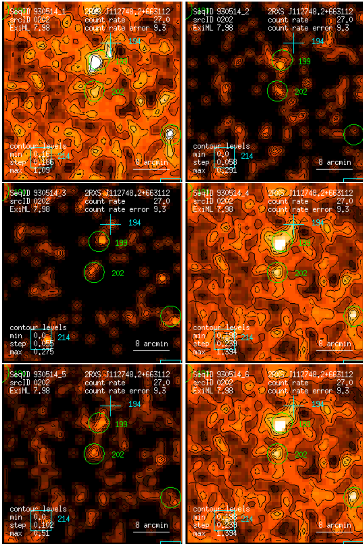
Figure 202: RASS 930514: detection 0202: band rate images, Gaussian filter: (1) PSPC channels 11 – 41, (2) 52 – 90, (3) 91 – 201, (4) 11 – 235, (5) 52 – 201, (6) 11 – 201. Broad band rates in counts/ks. Band rate contour levels in counts/ks/arcmin 2 .
