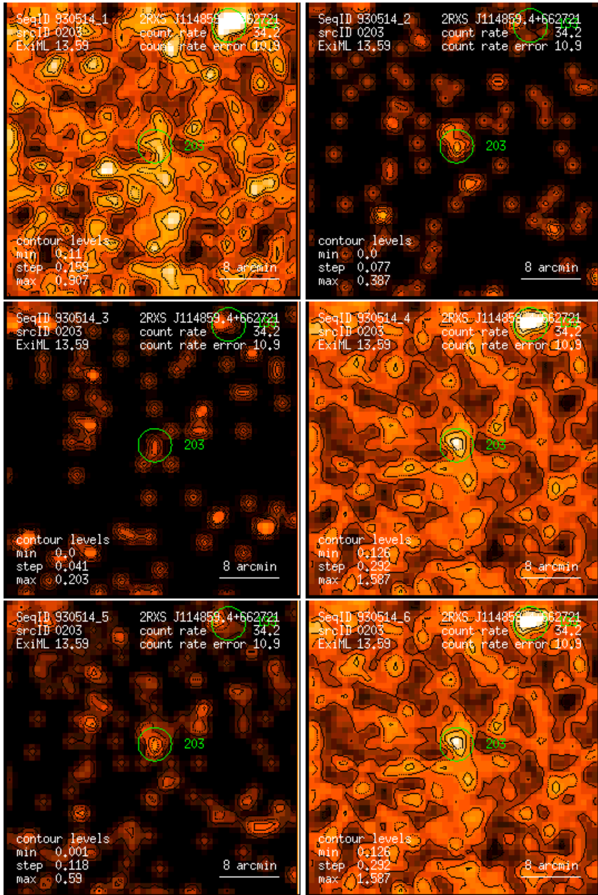
Figure 203: RASS 930514: detection 0203: band rate images, Gaussian filter: (1) PSPC channels 11 – 41, (2) 52 – 90, (3) 91 – 201, (4) 11 – 235, (5) 52 – 201, (6) 11 – 201. Broad band rates in counts/ks. Band rate contour levels in counts/ks/arcmin 2 .
