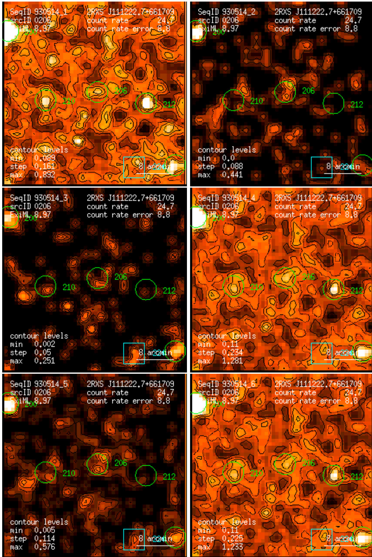
Figure 206: RASS 930514: detection 0206: band rate images, Gaussian filter: (1) PSPC channels 11 – 41, (2) 52 – 90, (3) 91 – 201, (4) 11 – 235, (5) 52 – 201, (6) 11 – 201. Broad band rates in counts/ks. Band rate contour levels in counts/ks/arcmin 2 .
