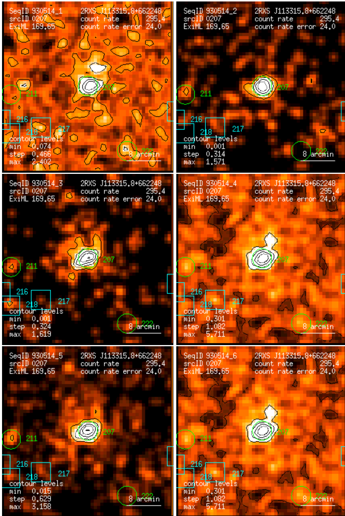
Figure 207: RASS 930514: detection 0207: band rate images, Gaussian filter: (1) PSPC channels 11 – 41, (2) 52 – 90, (3) 91 – 201, (4) 11 – 235, (5) 52 – 201, (6) 11 – 201. Broad band rates in counts/ks. Band rate contour levels in counts/ks/arcmin 2 .
