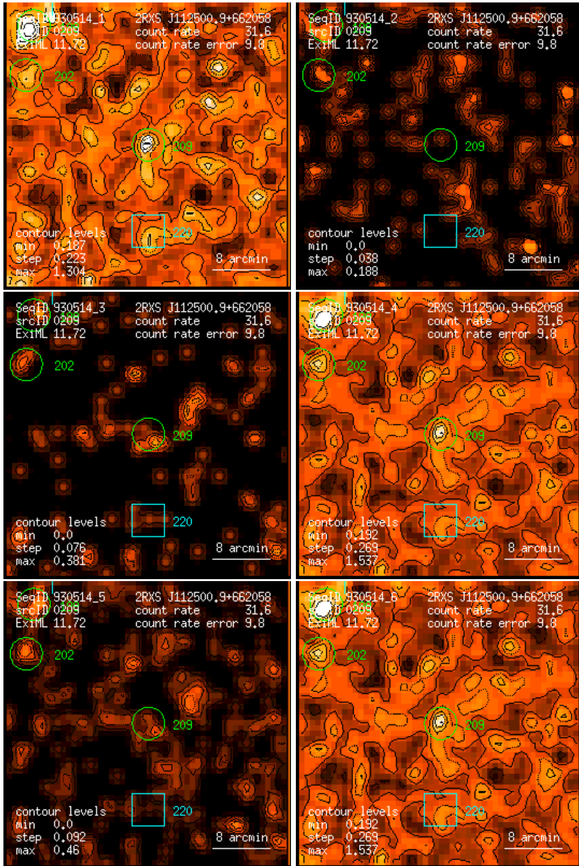
Figure 209: RASS 930514: detection 0209: band rate images, Gaussian filter: (1) PSPC channels 11 – 41, (2) 52 – 90, (3) 91 – 201, (4) 11 – 235, (5) 52 – 201, (6) 11 – 201. Broad band rates in counts/ks. Band rate contour levels in counts/ks/arcmin 2 .
