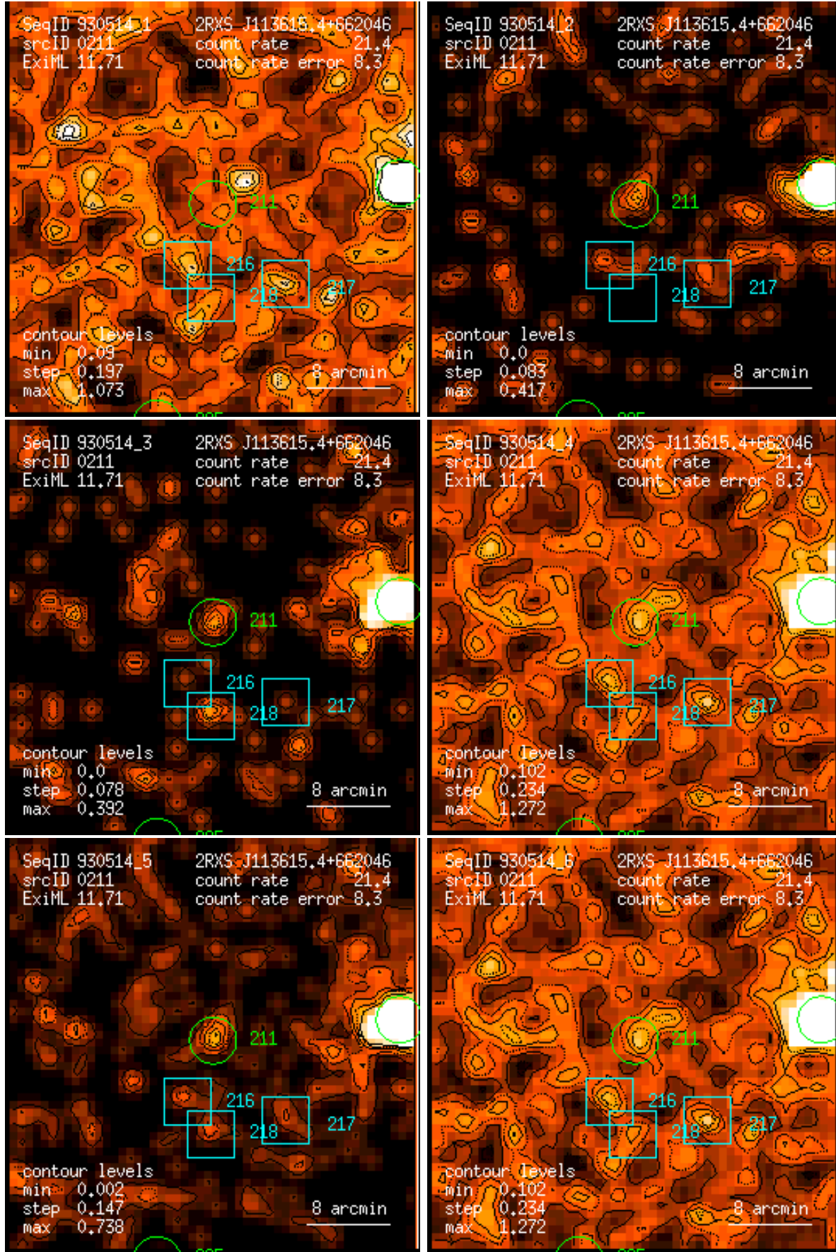
Figure 211: RASS 930514: detection 0211: band rate images, Gaussian filter: (1) PSPC channels 11 – 41, (2) 52 – 90, (3) 91 – 201, (4) 11 – 235, (5) 52 – 201, (6) 11 – 201. Broad band rates in counts/ks. Band rate contour levels in counts/ks/arcmin 2 .
