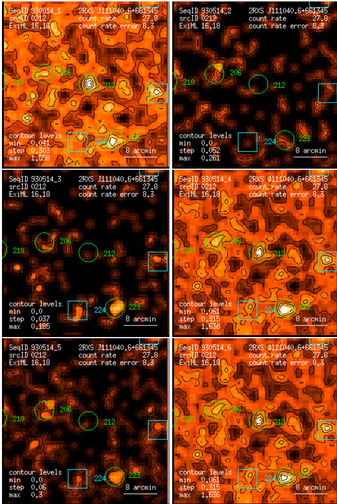
Figure 212: RASS 930514: detection 0212: band rate images, Gaussian filter: (1) PSPC channels 11 – 41, (2) 52 – 90, (3) 91 – 201, (4) 11 – 235, (5) 52 – 201, (6) 11 – 201. Broad band rates in counts/ks. Band rate contour levels in counts/ks/arcmin 2 .
