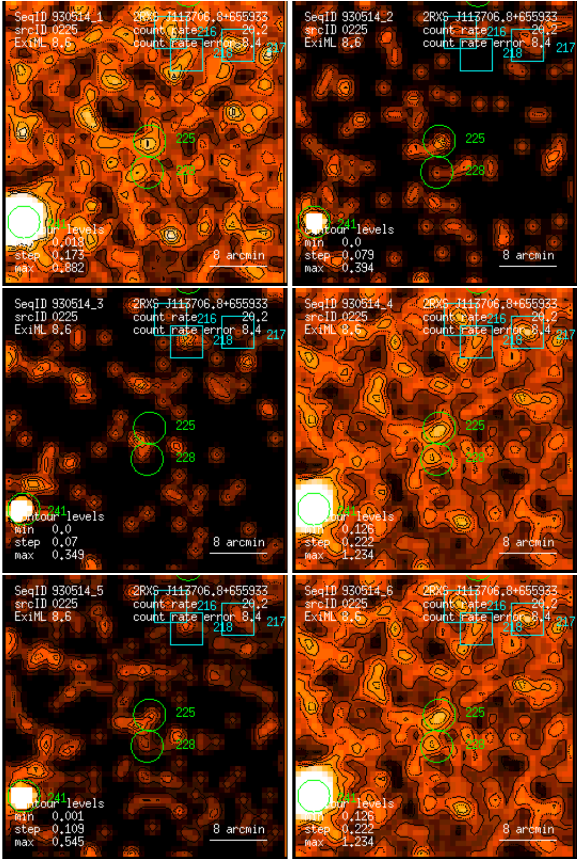
Figure 225: RASS 930514: detection 0225: band rate images, Gaussian filter: (1) PSPC channels 11 – 41, (2) 52 – 90, (3) 91 – 201, (4) 11 – 235, (5) 52 – 201, (6) 11 – 201. Broad band rates in counts/ks. Band rate contour levels in counts/ks/arcmin 2 .
