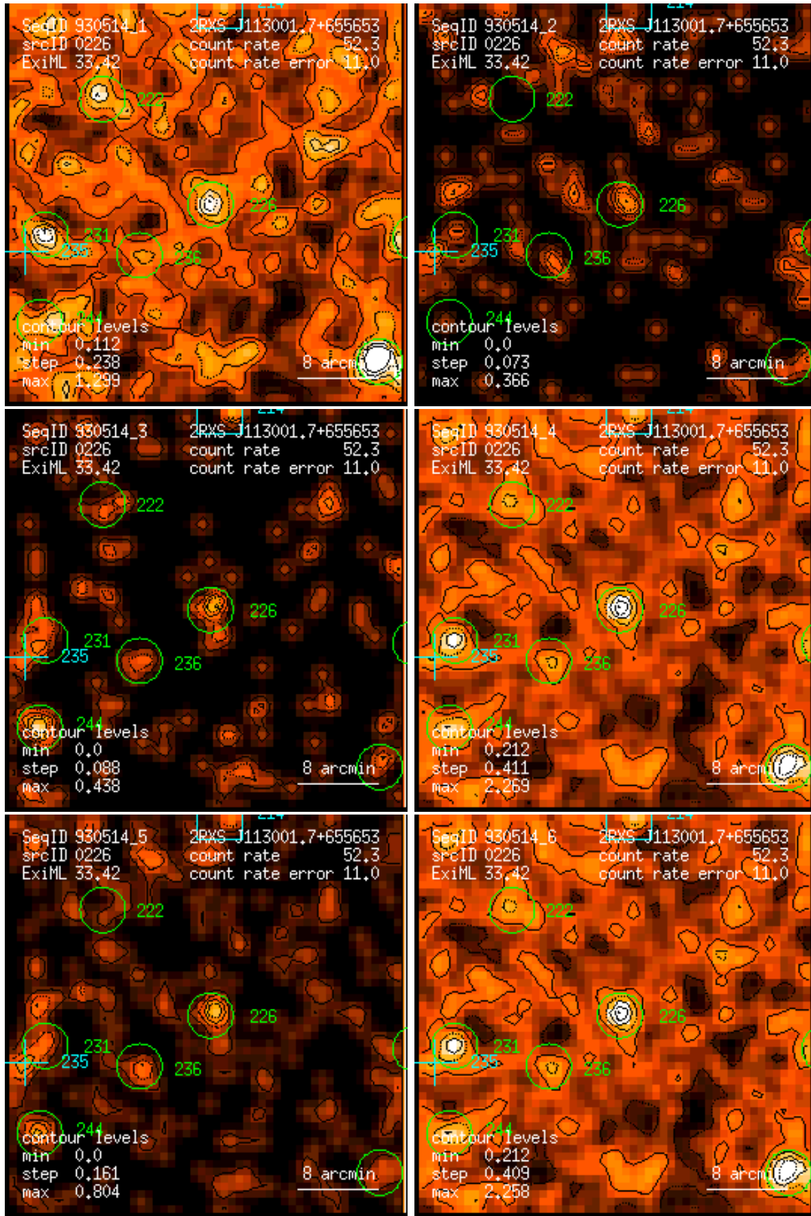
Figure 226: RASS 930514: detection 0226: band rate images, Gaussian filter: (1) PSPC channels 11 – 41, (2) 52 – 90, (3) 91 – 201, (4) 11 – 235, (5) 52 – 201, (6) 11 – 201. Broad band rates in counts/ks. Band rate contour levels in counts/ks/arcmin 2 .
