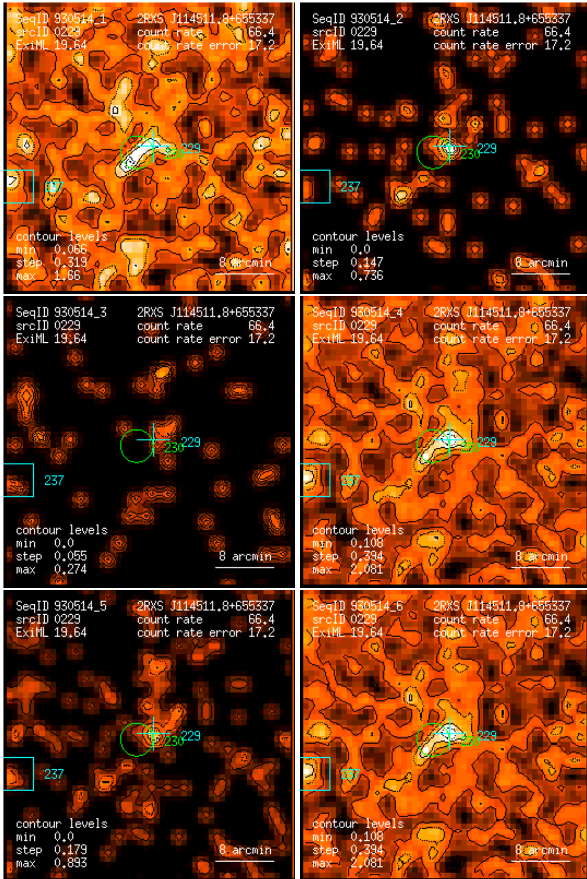
Figure 229: RASS 930514: detection 0229: band rate images, Gaussian filter: (1) PSPC channels 11 – 41, (2) 52 – 90, (3) 91 – 201, (4) 11 – 235, (5) 52 – 201, (6) 11 – 201. Broad band rates in counts/ks. Band rate contour levels in counts/ks/arcmin 2 .
