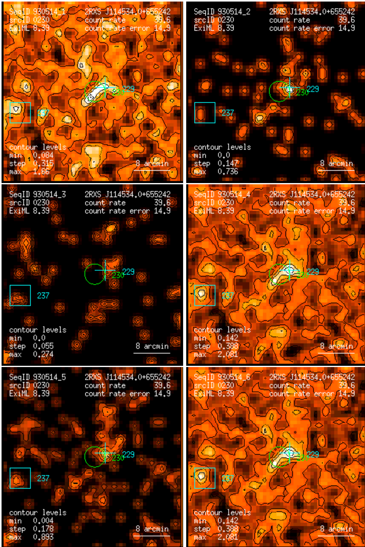
Figure 230: RASS 930514: detection 0230: band rate images, Gaussian filter: (1) PSPC channels 11 – 41, (2) 52 – 90, (3) 91 – 201, (4) 11 – 235, (5) 52 – 201, (6) 11 – 201. Broad band rates in counts/ks. Band rate contour levels in counts/ks/arcmin 2 .
