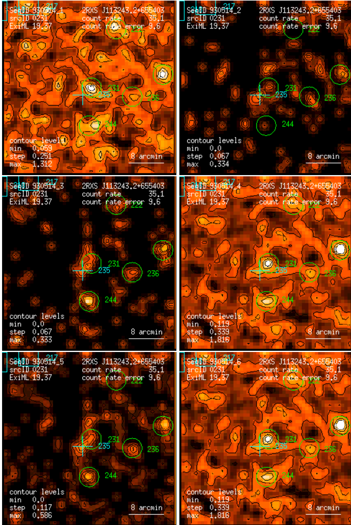
Figure 231: RASS 930514: detection 0231: band rate images, Gaussian filter: (1) PSPC channels 11 – 41, (2) 52 – 90, (3) 91 – 201, (4) 11 – 235, (5) 52 – 201, (6) 11 – 201. Broad band rates in counts/ks. Band rate contour levels in counts/ks/arcmin 2 .
