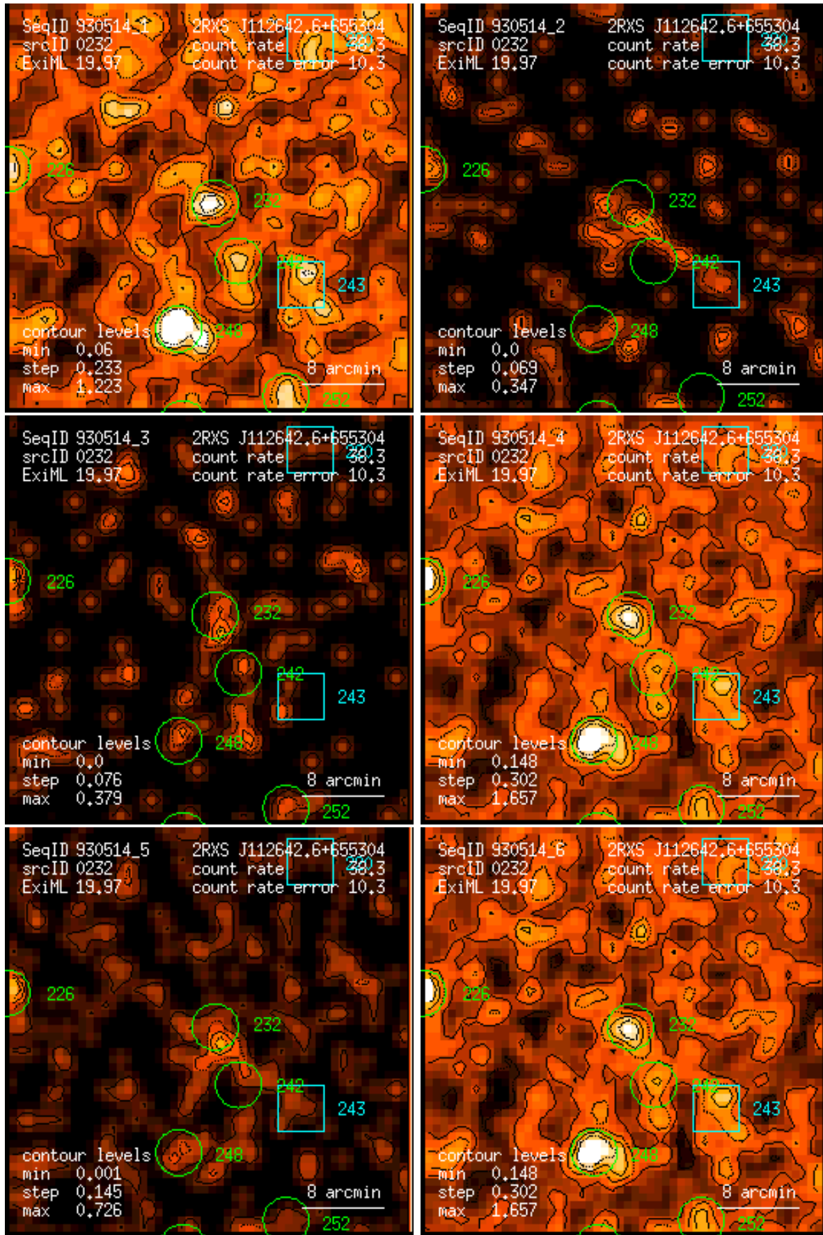
Figure 232: RASS 930514: detection 0232: band rate images, Gaussian filter: (1) PSPC channels 11 – 41, (2) 52 – 90, (3) 91 – 201, (4) 11 – 235, (5) 52 – 201, (6) 11 – 201. Broad band rates in counts/ks. Band rate contour levels in counts/ks/arcmin 2 .
