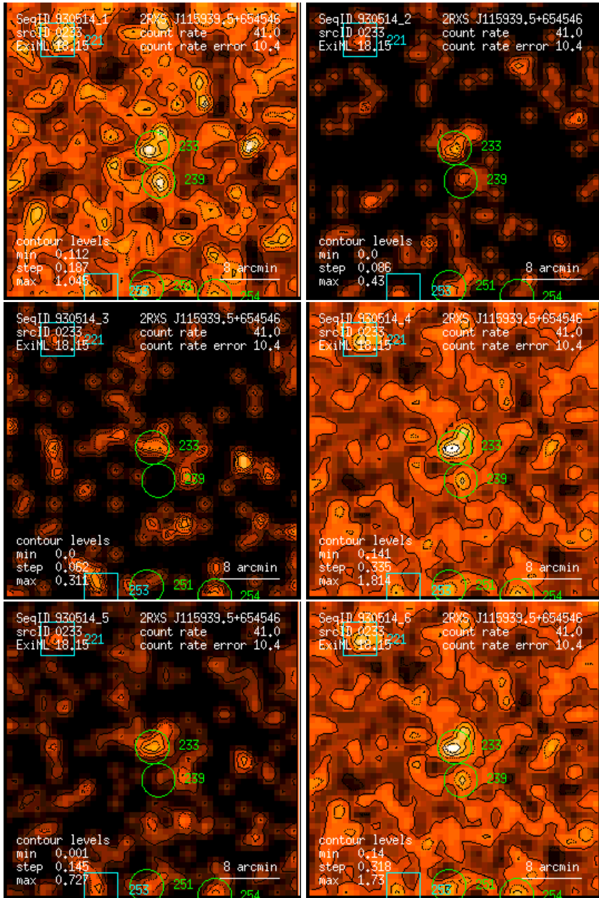
Figure 233: RASS 930514: detection 0233: band rate images, Gaussian filter: (1) PSPC channels 11 – 41, (2) 52 – 90, (3) 91 – 201, (4) 11 – 235, (5) 52 – 201, (6) 11 – 201. Broad band rates in counts/ks. Band rate contour levels in counts/ks/arcmin 2 .
