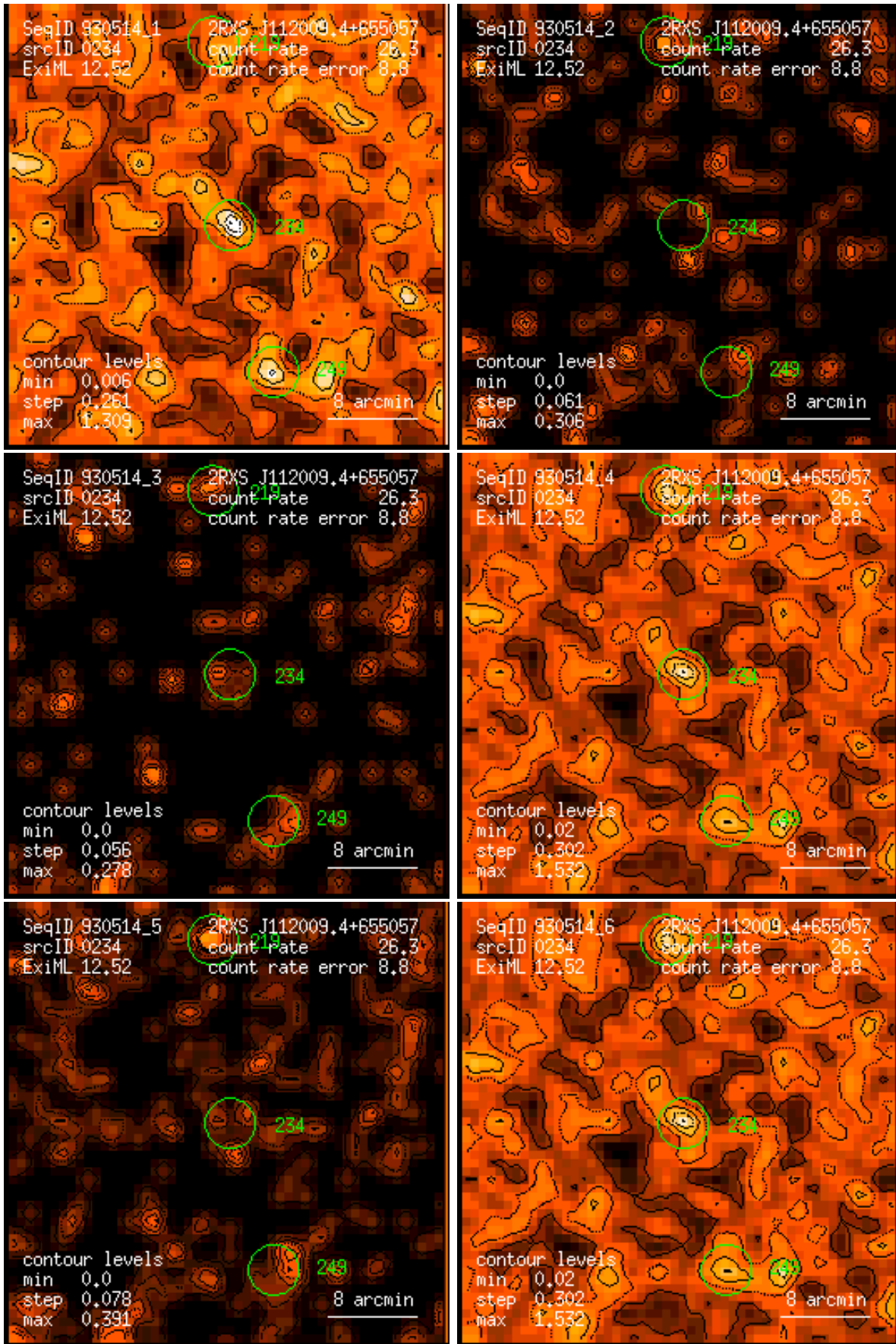
Figure 234: RASS 930514: detection 0234: band rate images, Gaussian filter: (1) PSPC channels 11 – 41, (2) 52 – 90, (3) 91 – 201, (4) 11 – 235, (5) 52 – 201, (6) 11 – 201. Broad band rates in counts/ks. Band rate contour levels in counts/ks/arcmin 2 .
