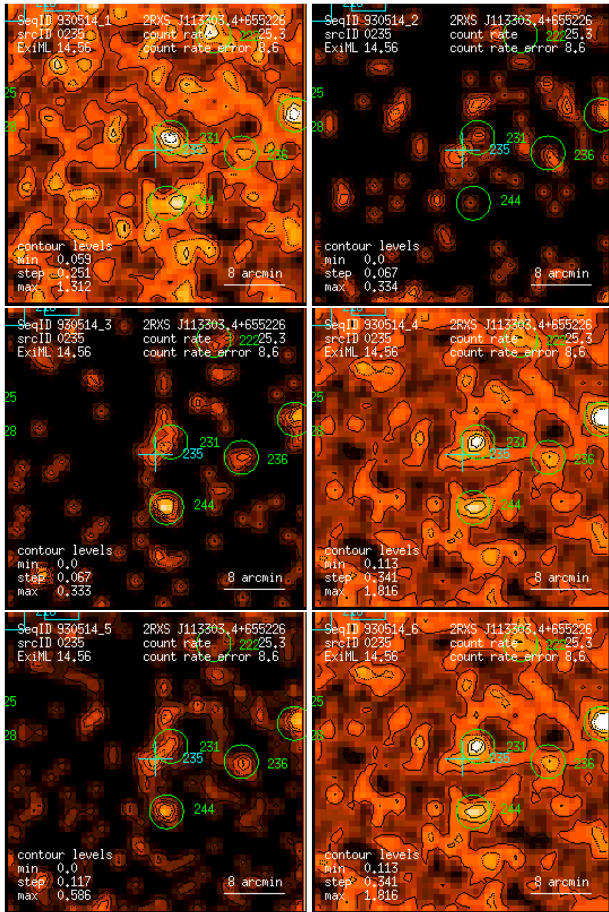
Figure 235: RASS 930514: detection 0235: band rate images, Gaussian filter: (1) PSPC channels 11 – 41, (2) 52 – 90, (3) 91 – 201, (4) 11 – 235, (5) 52 – 201, (6) 11 – 201. Broad band rates in counts/ks. Band rate contour levels in counts/ks/arcmin 2 .
