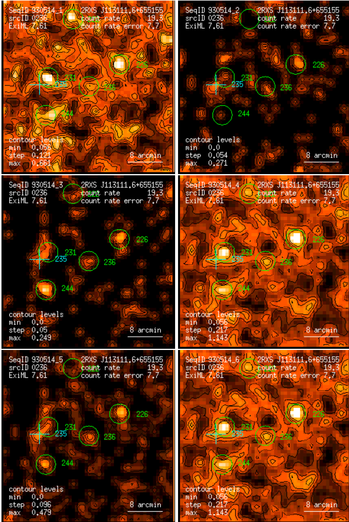
Figure 236: RASS 930514: detection 0236: band rate images, Gaussian filter: (1) PSPC channels 11 – 41, (2) 52 – 90, (3) 91 – 201, (4) 11 – 235, (5) 52 – 201, (6) 11 – 201. Broad band rates in counts/ks. Band rate contour levels in counts/ks/arcmin 2 .
