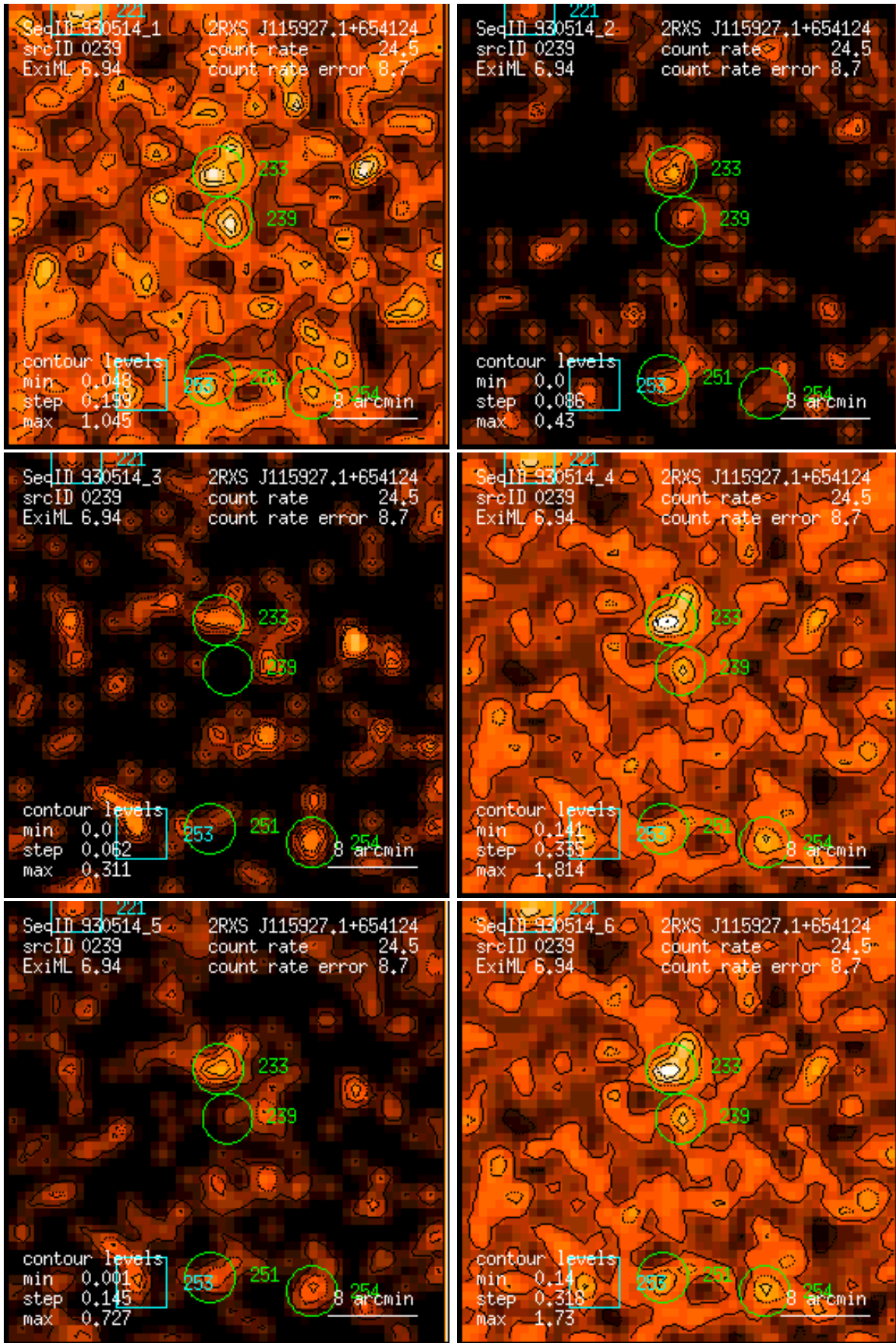
Figure 239: RASS 930514: detection 0239: band rate images, Gaussian filter: (1) PSPC channels 11 – 41, (2) 52 – 90, (3) 91 – 201, (4) 11 – 235, (5) 52 – 201, (6) 11 – 201. Broad band rates in counts/ks. Band rate contour levels in counts/ks/arcmin 2 .
