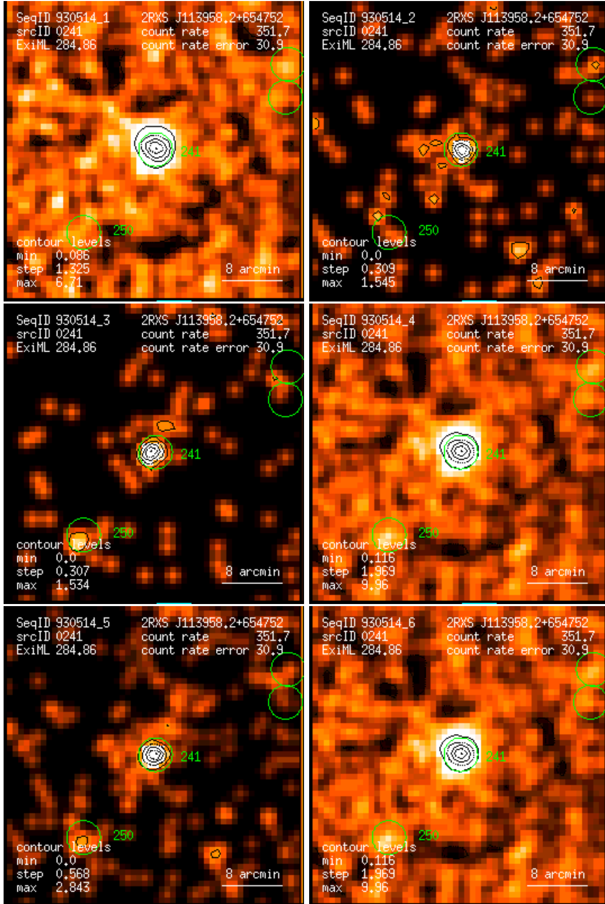
Figure 241: RASS 930514: detection 0241: band rate images, Gaussian filter: (1) PSPC channels 11 – 41, (2) 52 – 90, (3) 91 – 201, (4) 11 – 235, (5) 52 – 201, (6) 11 – 201. Broad band rates in counts/ks. Band rate contour levels in counts/ks/arcmin 2 .
