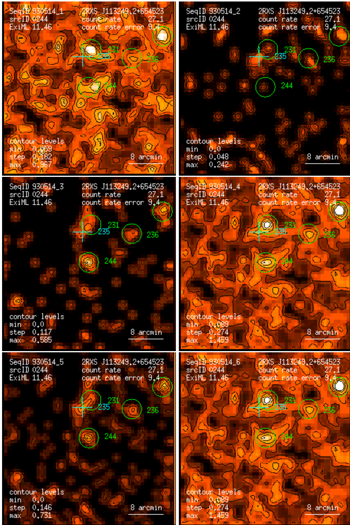
Figure 244: RASS 930514: detection 0244: band rate images, Gaussian filter: (1) PSPC channels 11 – 41, (2) 52 – 90, (3) 91 – 201, (4) 11 – 235, (5) 52 – 201, (6) 11 – 201. Broad band rates in counts/ks. Band rate contour levels in counts/ks/arcmin 2 .
