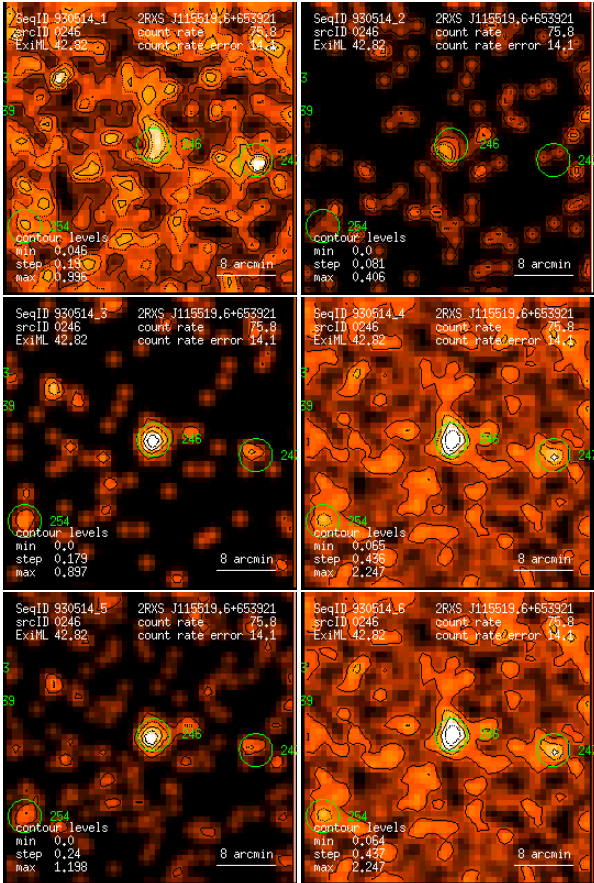
Figure 246: RASS 930514: detection 0246: band rate images, Gaussian filter: (1) PSPC channels 11 – 41, (2) 52 – 90, (3) 91 – 201, (4) 11 – 235, (5) 52 – 201, (6) 11 – 201. Broad band rates in counts/ks. Band rate contour levels in counts/ks/arcmin 2 .
