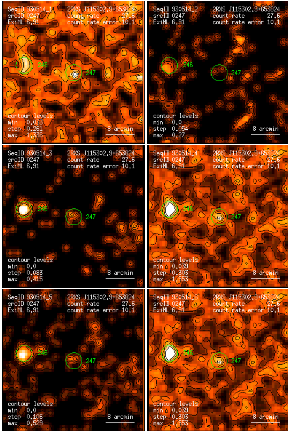
Figure 247: RASS 930514: detection 0247: band rate images, Gaussian filter: (1) PSPC channels 11 – 41, (2) 52 – 90, (3) 91 – 201, (4) 11 – 235, (5) 52 – 201, (6) 11 – 201. Broad band rates in counts/ks. Band rate contour levels in counts/ks/arcmin 2 .
