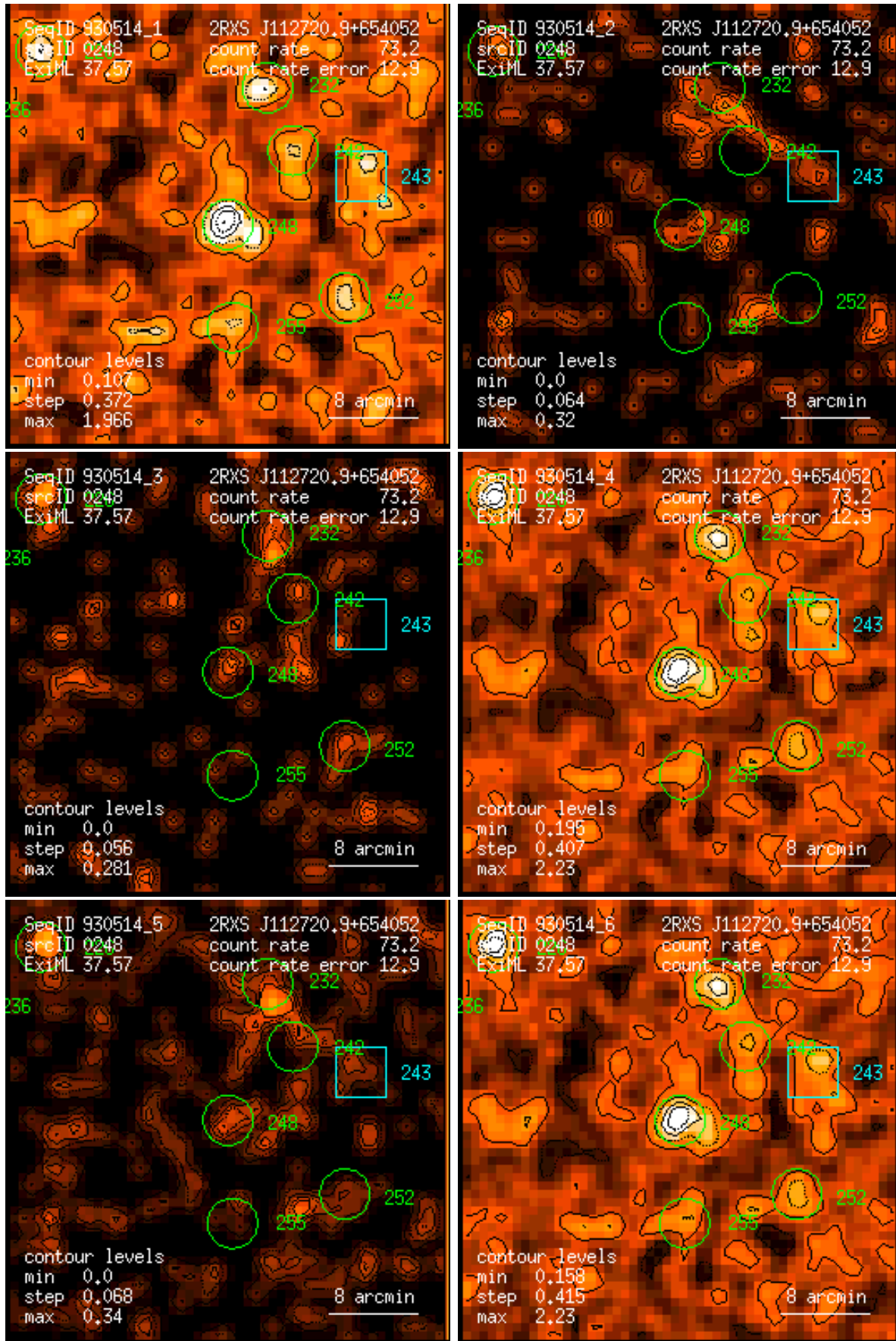
Figure 248: RASS 930514: detection 0248: band rate images, Gaussian filter: (1) PSPC channels 11 – 41, (2) 52 – 90, (3) 91 – 201, (4) 11 – 235, (5) 52 – 201, (6) 11 – 201. Broad band rates in counts/ks. Band rate contour levels in counts/ks/arcmin 2 .
