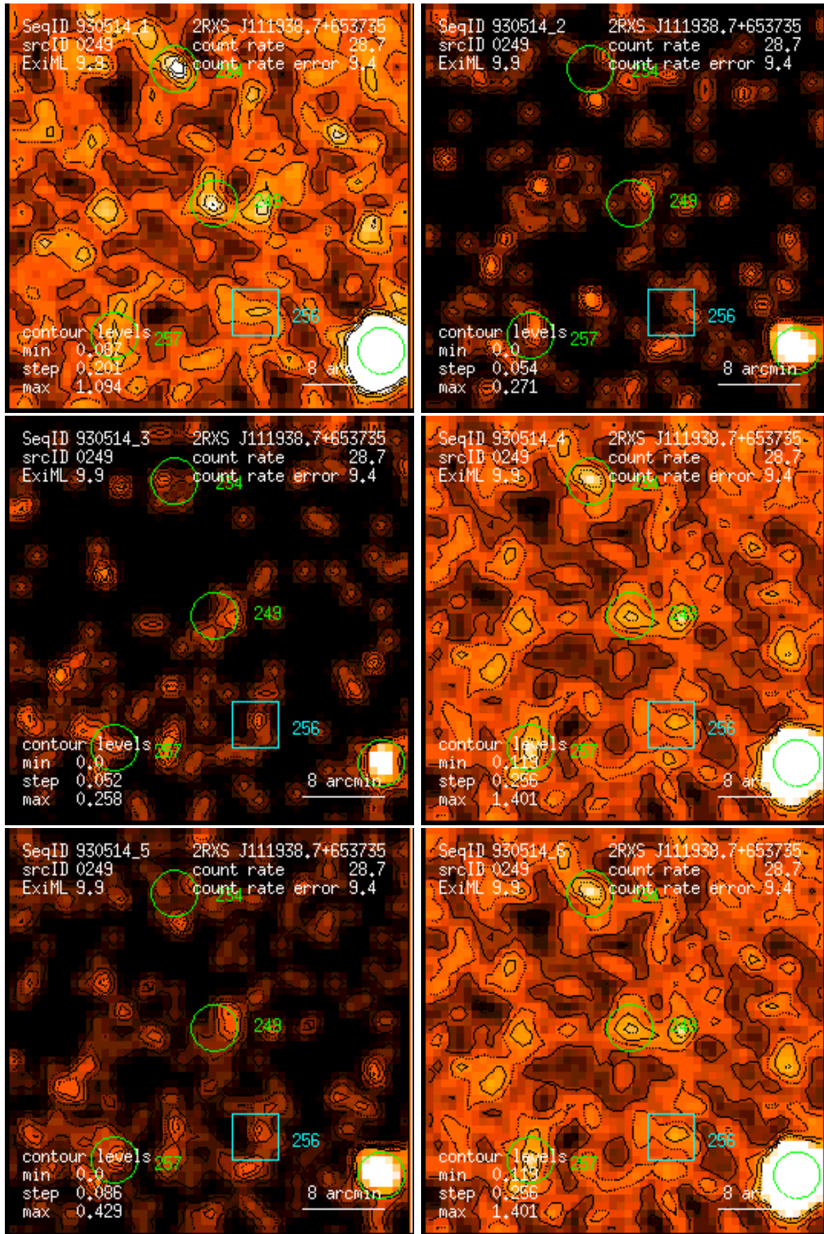
Figure 249: RASS 930514: detection 0249: band rate images, Gaussian filter: (1) PSPC channels 11 – 41, (2) 52 – 90, (3) 91 – 201, (4) 11 – 235, (5) 52 – 201, (6) 11 – 201. Broad band rates in counts/ks. Band rate contour levels in counts/ks/arcmin 2 .
