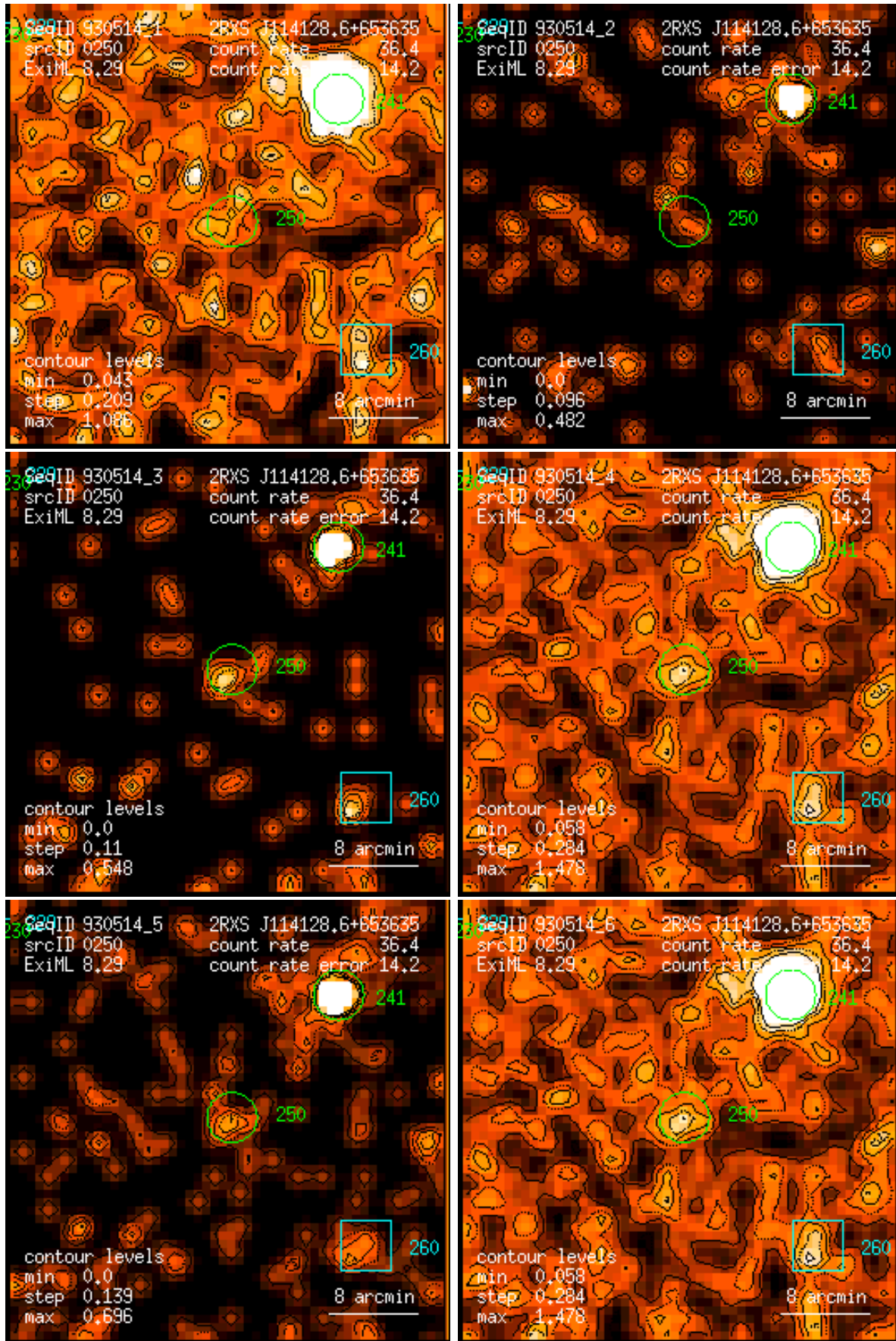
Figure 250: RASS 930514: detection 0250: band rate images, Gaussian filter: (1) PSPC channels 11 – 41, (2) 52 – 90, (3) 91 – 201, (4) 11 – 235, (5) 52 – 201, (6) 11 – 201. Broad band rates in counts/ks. Band rate contour levels in counts/ks/arcmin 2 .
