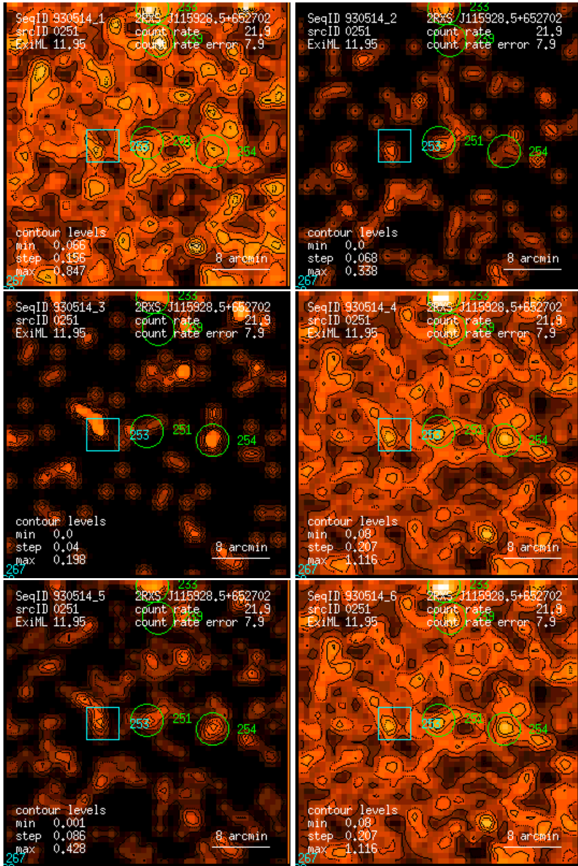
Figure 251: RASS 930514: detection 0251: band rate images, Gaussian filter: (1) PSPC channels 11 – 41, (2) 52 – 90, (3) 91 – 201, (4) 11 – 235, (5) 52 – 201, (6) 11 – 201. Broad band rates in counts/ks. Band rate contour levels in counts/ks/arcmin 2 .
