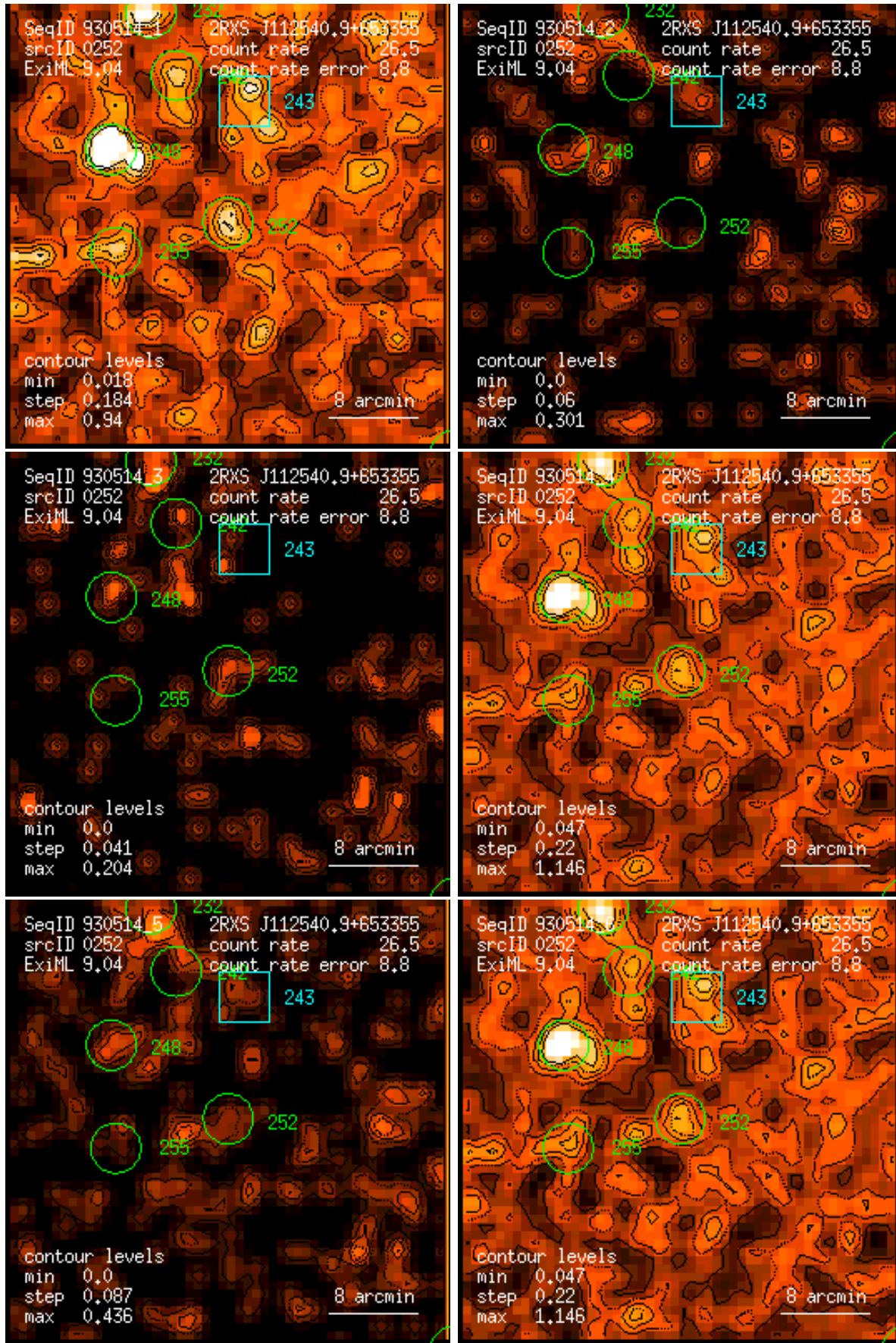
Figure 252: RASS 930514: detection 0252: band rate images, Gaussian filter: (1) PSPC channels 11 – 41, (2) 52 – 90, (3) 91 – 201, (4) 11 – 235, (5) 52 – 201, (6) 11 – 201. Broad band rates in counts/ks. Band rate contour levels in counts/ks/arcmin 2 .
