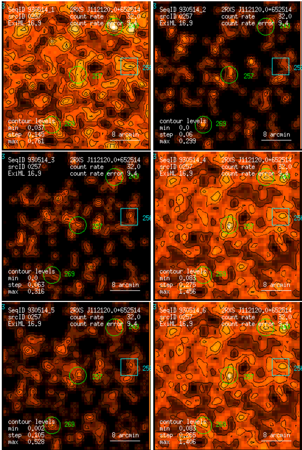
Figure 257: RASS 930514: detection 0257: band rate images, Gaussian filter: (1) PSPC channels 11 – 41, (2) 52 – 90, (3) 91 – 201, (4) 11 – 235, (5) 52 – 201, (6) 11 – 201. Broad band rates in counts/ks. Band rate contour levels in counts/ks/arcmin 2 .
