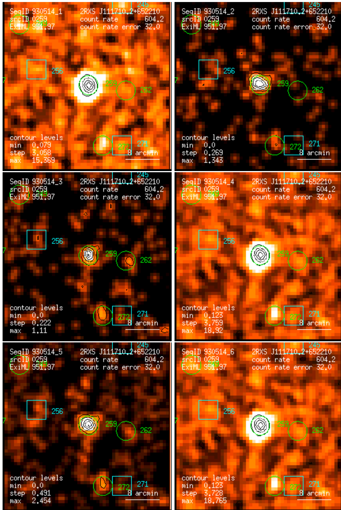
Figure 259: RASS 930514: detection 0259: band rate images, Gaussian filter: (1) PSPC channels 11 – 41, (2) 52 – 90, (3) 91 – 201, (4) 11 – 235, (5) 52 – 201, (6) 11 – 201. Broad band rates in counts/ks. Band rate contour levels in counts/ks/arcmin 2 .
