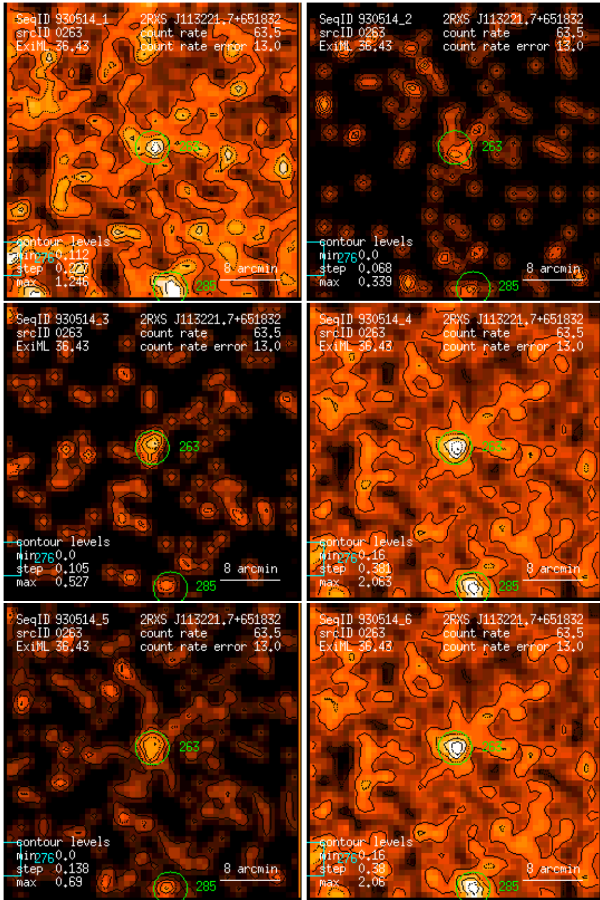
Figure 263: RASS 930514: detection 0263: band rate images, Gaussian filter: (1) PSPC channels 11 – 41, (2) 52 – 90, (3) 91 – 201, (4) 11 – 235, (5) 52 – 201, (6) 11 – 201. Broad band rates in counts/ks. Band rate contour levels in counts/ks/arcmin 2 .
