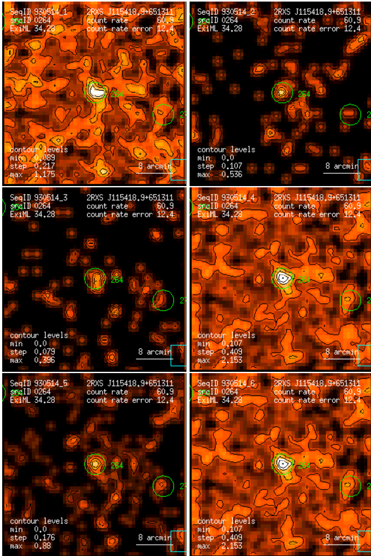
Figure 264: RASS 930514: detection 0264: band rate images, Gaussian filter: (1) PSPC channels 11 – 41, (2) 52 – 90, (3) 91 – 201, (4) 11 – 235, (5) 52 – 201, (6) 11 – 201. Broad band rates in counts/ks. Band rate contour levels in counts/ks/arcmin 2 .
