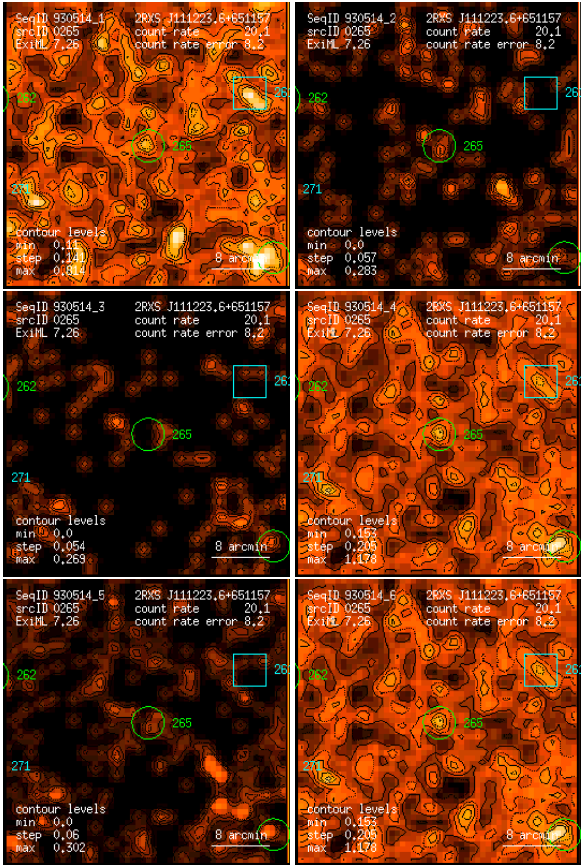
Figure 265: RASS 930514: detection 0265: band rate images, Gaussian filter: (1) PSPC channels 11 – 41, (2) 52 – 90, (3) 91 – 201, (4) 11 – 235, (5) 52 – 201, (6) 11 – 201. Broad band rates in counts/ks. Band rate contour levels in counts/ks/arcmin 2 .
