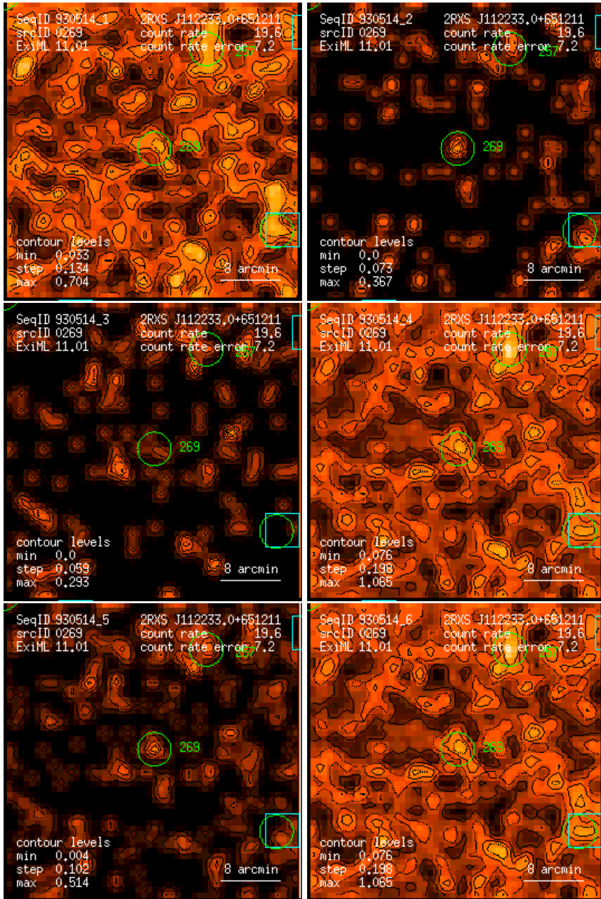
Figure 269: RASS 930514: detection 0269: band rate images, Gaussian filter: (1) PSPC channels 11 – 41, (2) 52 – 90, (3) 91 – 201, (4) 11 – 235, (5) 52 – 201, (6) 11 – 201. Broad band rates in counts/ks. Band rate contour levels in counts/ks/arcmin 2 .
