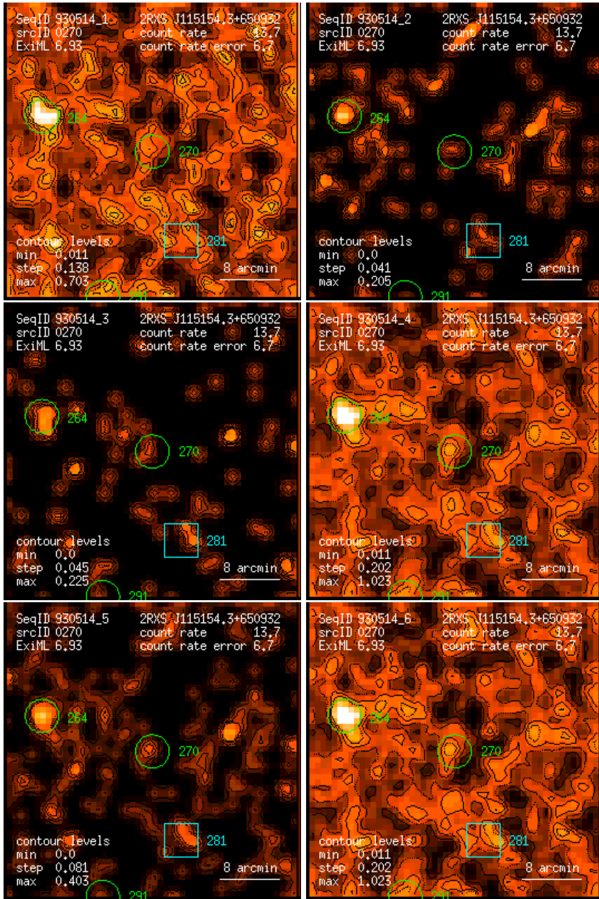
Figure 270: RASS 930514: detection 0270: band rate images, Gaussian filter: (1) PSPC channels 11 – 41, (2) 52 – 90, (3) 91 – 201, (4) 11 – 235, (5) 52 – 201, (6) 11 – 201. Broad band rates in counts/ks. Band rate contour levels in counts/ks/arcmin 2 .
