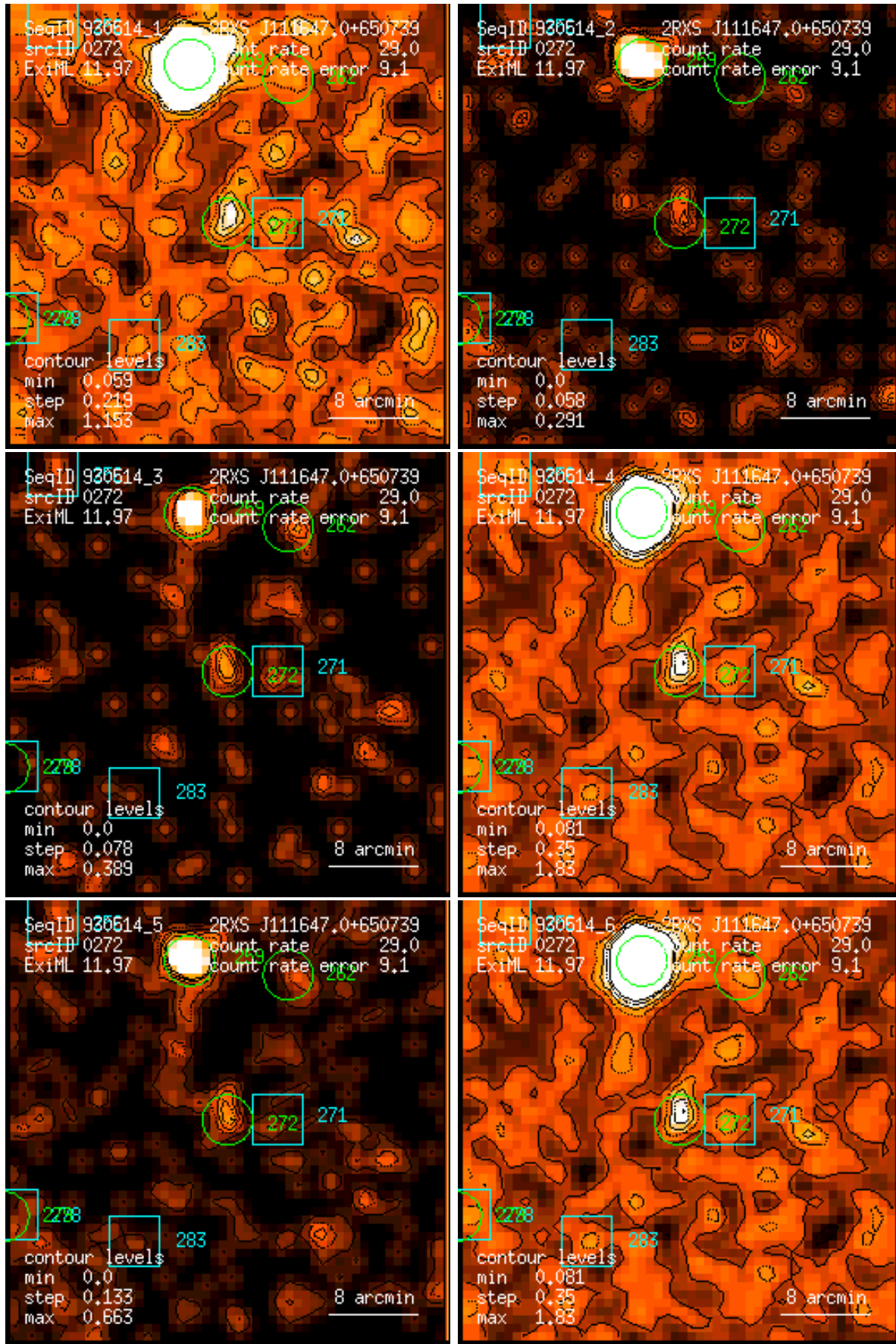
Figure 272: RASS 930514: detection 0272: band rate images, Gaussian filter: (1) PSPC channels 11 – 41, (2) 52 – 90, (3) 91 – 201, (4) 11 – 235, (5) 52 – 201, (6) 11 – 201. Broad band rates in counts/ks. Band rate contour levels in counts/ks/arcmin 2 .
