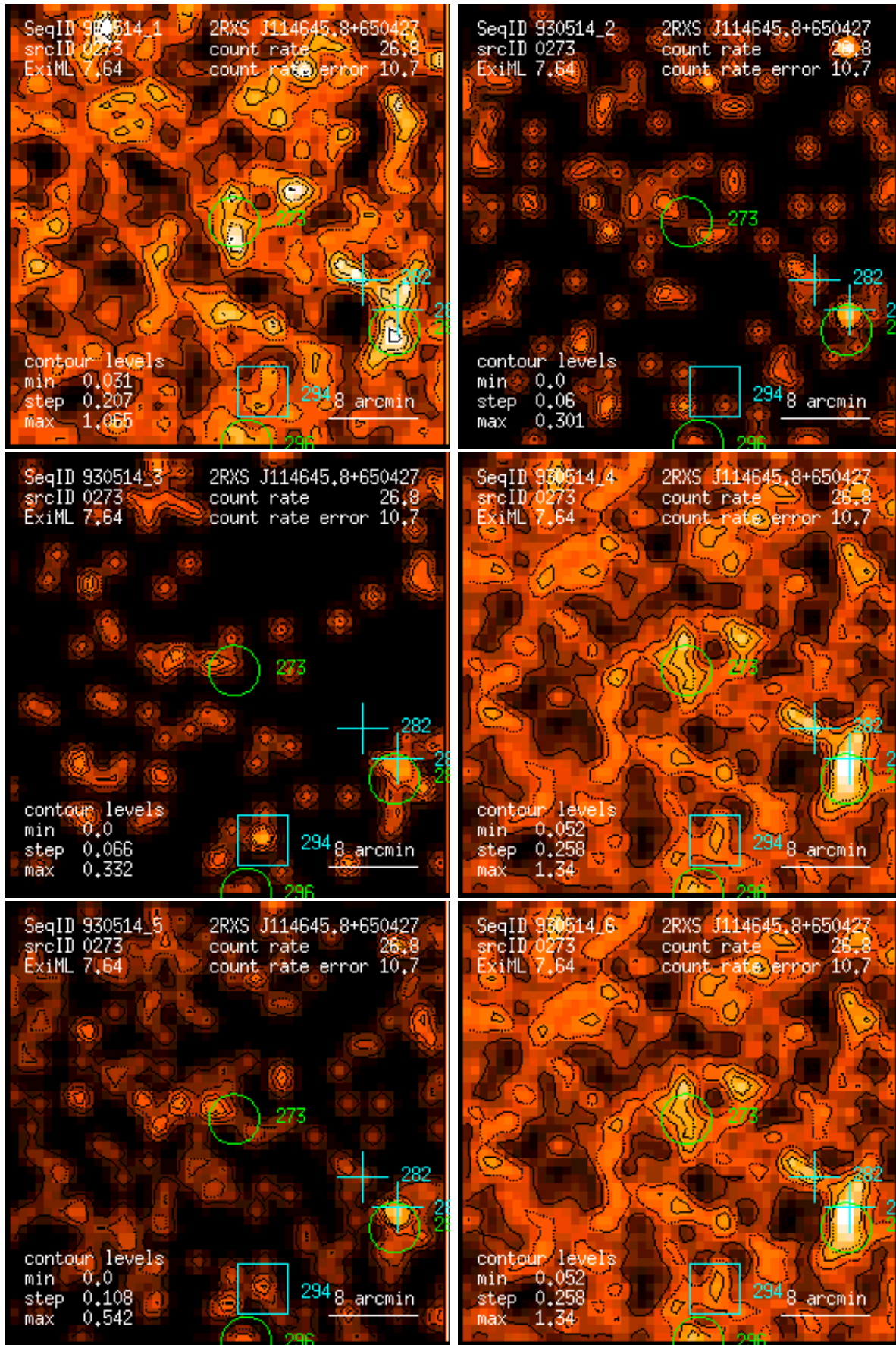
Figure 273: RASS 930514: detection 0273: band rate images, Gaussian filter: (1) PSPC channels 11 – 41, (2) 52 – 90, (3) 91 – 201, (4) 11 – 235, (5) 52 – 201, (6) 11 – 201. Broad band rates in counts/ks. Band rate contour levels in counts/ks/arcmin 2 .
