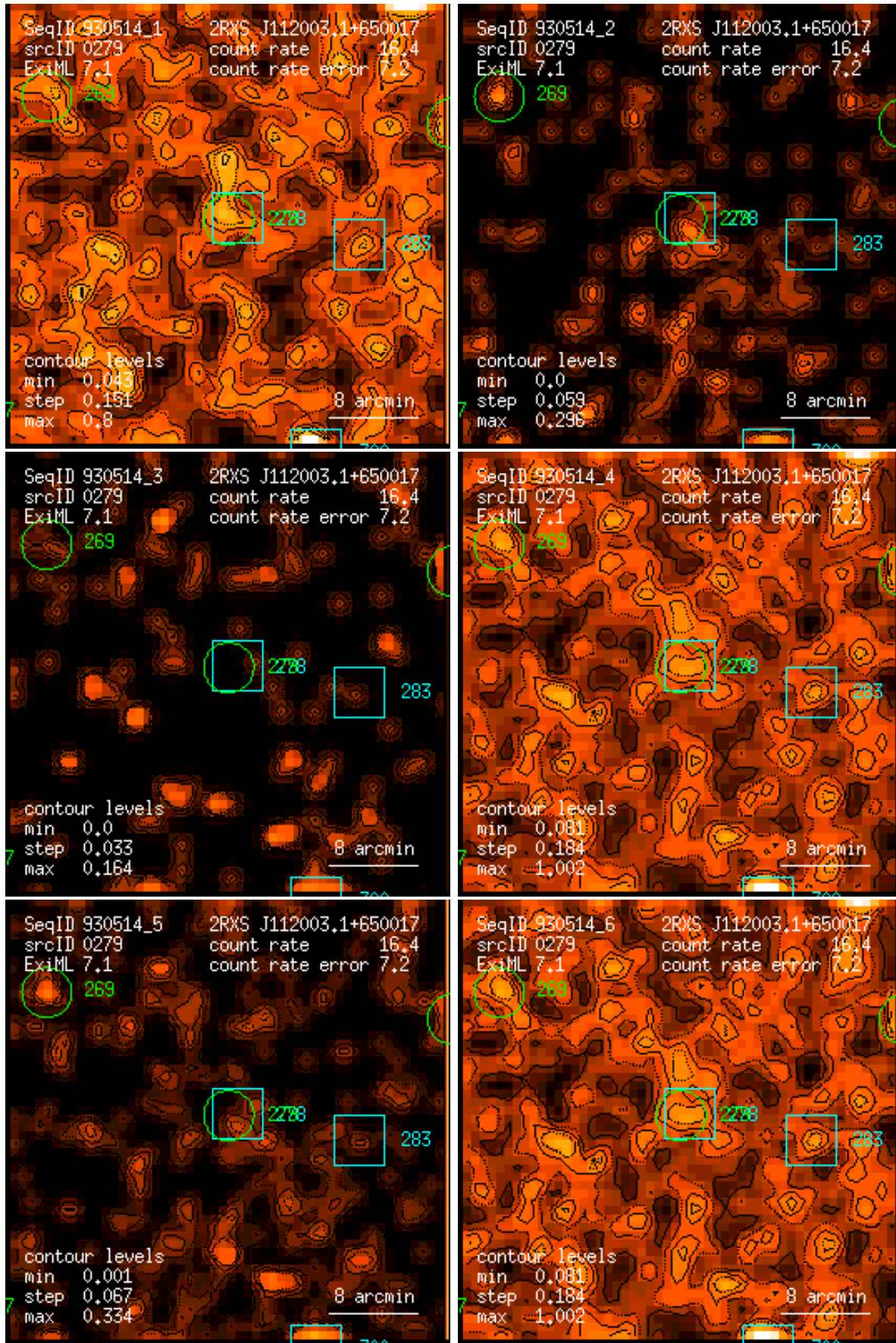
Figure 279: RASS 930514: detection 0279: band rate images, Gaussian filter: (1) PSPC channels 11 – 41, (2) 52 – 90, (3) 91 – 201, (4) 11 – 235, (5) 52 – 201, (6) 11 – 201. Broad band rates in counts/ks. Band rate contour levels in counts/ks/arcmin 2 .
