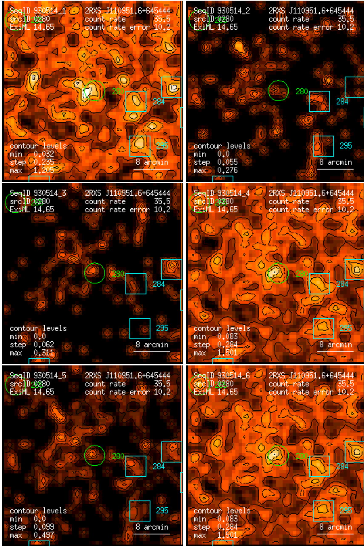
Figure 280: RASS 930514: detection 0280: band rate images, Gaussian filter: (1) PSPC channels 11 – 41, (2) 52 – 90, (3) 91 – 201, (4) 11 – 235, (5) 52 – 201, (6) 11 – 201. Broad band rates in counts/ks. Band rate contour levels in counts/ks/arcmin 2 .
