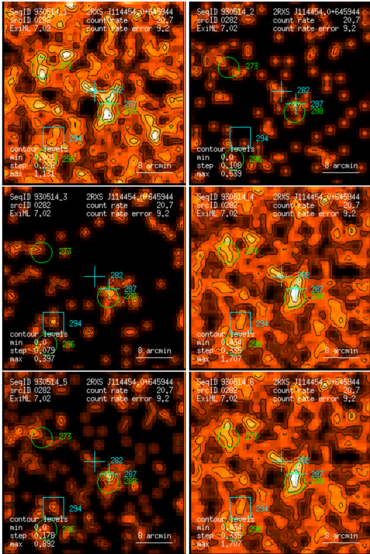
Figure 282: RASS 930514: detection 0282: band rate images, Gaussian filter: (1) PSPC channels 11 – 41, (2) 52 – 90, (3) 91 – 201, (4) 11 – 235, (5) 52 – 201, (6) 11 – 201. Broad band rates in counts/ks. Band rate contour levels in counts/ks/arcmin 2 .
