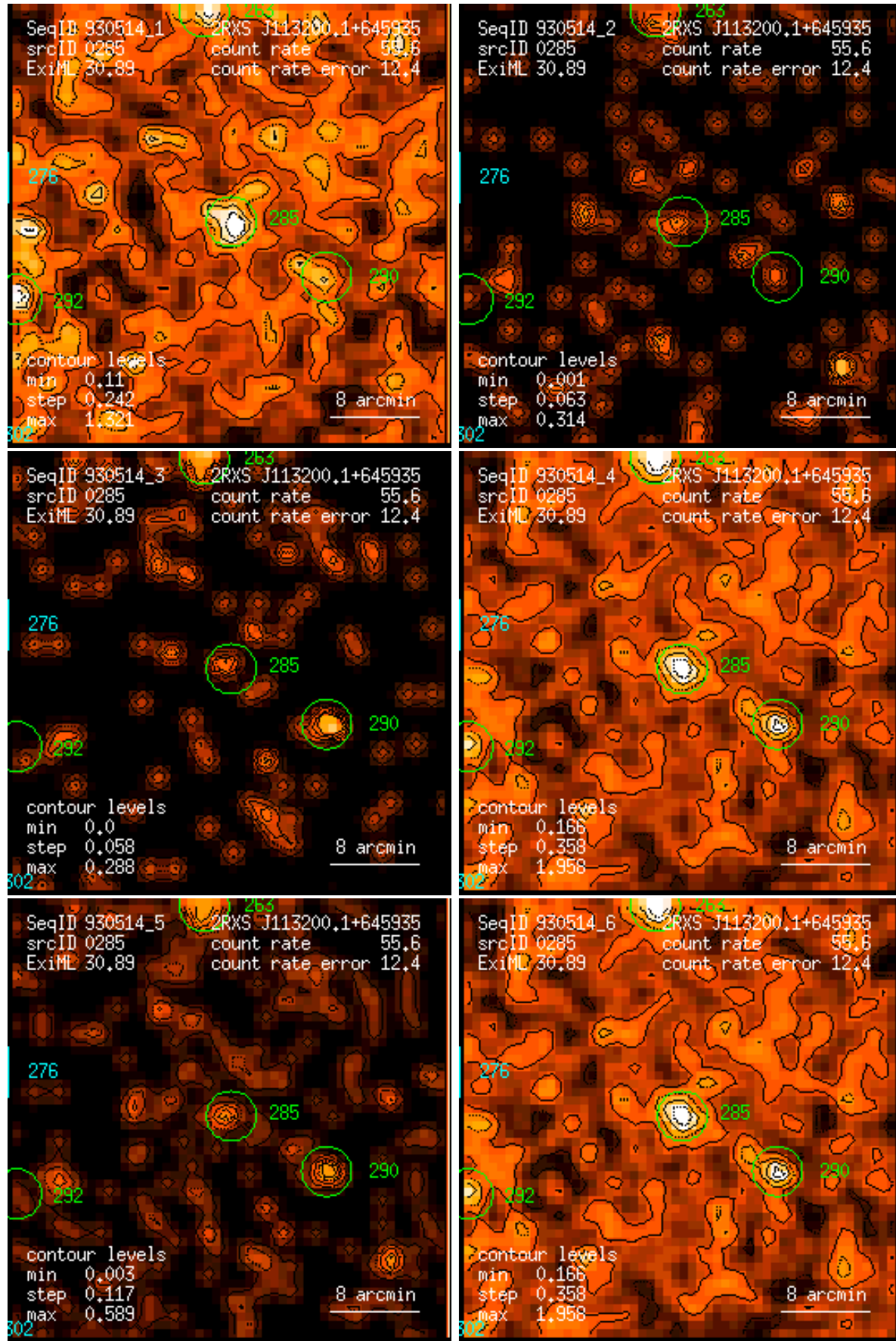
Figure 285: RASS 930514: detection 0285: band rate images, Gaussian filter: (1) PSPC channels 11 – 41, (2) 52 – 90, (3) 91 – 201, (4) 11 – 235, (5) 52 – 201, (6) 11 – 201. Broad band rates in counts/ks. Band rate contour levels in counts/ks/arcmin 2 .
