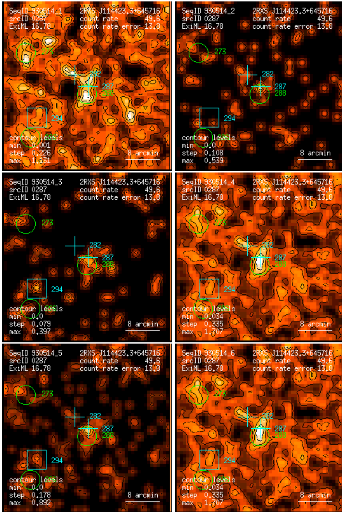
Figure 287: RASS 930514: detection 0287: band rate images, Gaussian filter: (1) PSPC channels 11 – 41, (2) 52 – 90, (3) 91 – 201, (4) 11 – 235, (5) 52 – 201, (6) 11 – 201. Broad band rates in counts/ks. Band rate contour levels in counts/ks/arcmin 2 .
