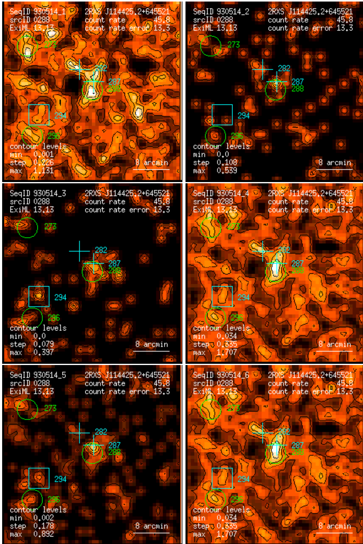
Figure 288: RASS 930514: detection 0288: band rate images, Gaussian filter: (1) PSPC channels 11 – 41, (2) 52 – 90, (3) 91 – 201, (4) 11 – 235, (5) 52 – 201, (6) 11 – 201. Broad band rates in counts/ks. Band rate contour levels in counts/ks/arcmin 2 .
