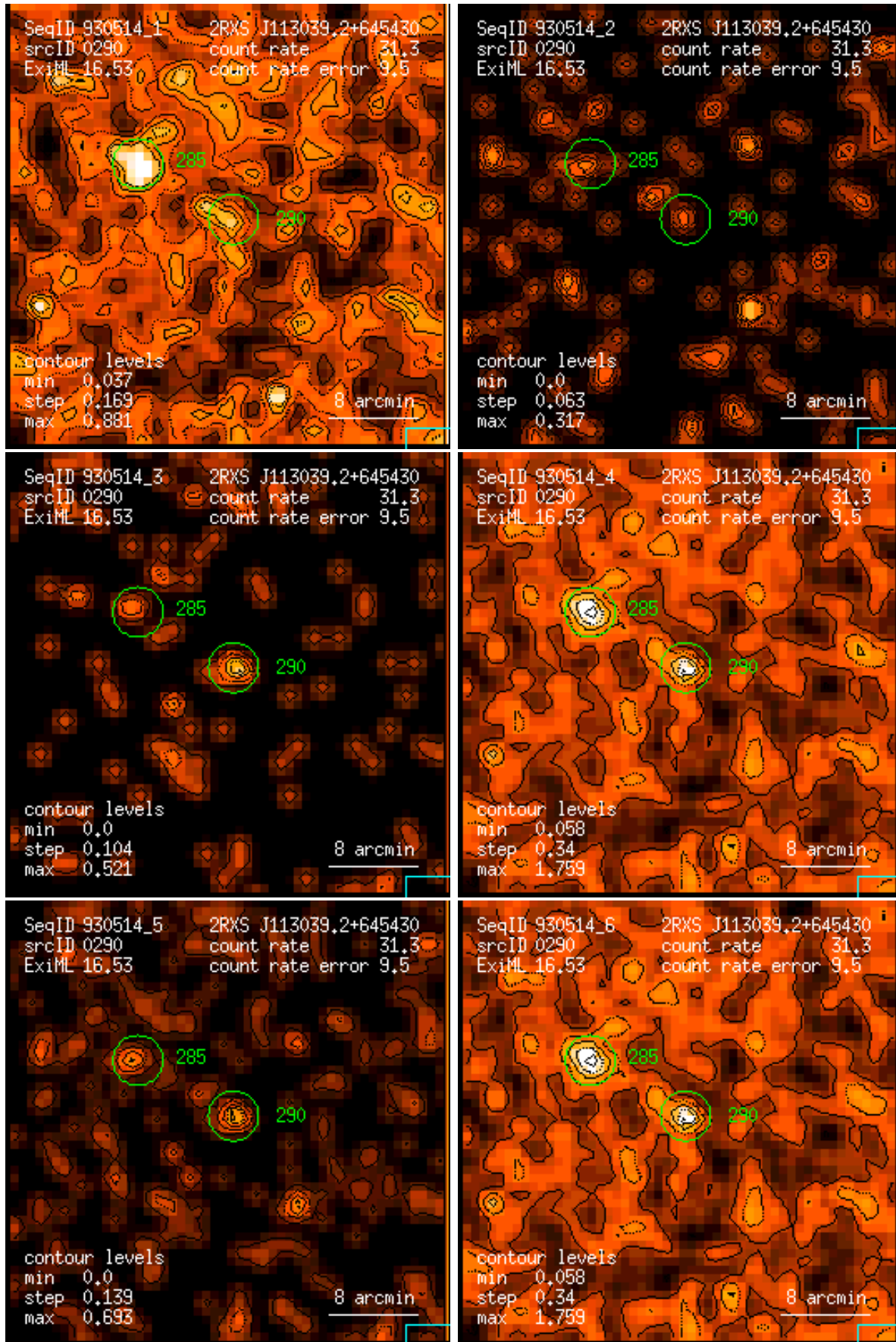
Figure 290: RASS 930514: detection 0290: band rate images, Gaussian filter: (1) PSPC channels 11 – 41, (2) 52 – 90, (3) 91 – 201, (4) 11 – 235, (5) 52 – 201, (6) 11 – 201. Broad band rates in counts/ks. Band rate contour levels in counts/ks/arcmin 2 .
