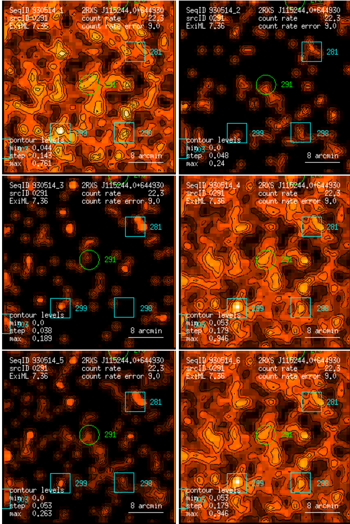
Figure 291: RASS 930514: detection 0291: band rate images, Gaussian filter: (1) PSPC channels 11 – 41, (2) 52 – 90, (3) 91 – 201, (4) 11 – 235, (5) 52 – 201, (6) 11 – 201. Broad band rates in counts/ks. Band rate contour levels in counts/ks/arcmin 2 .
