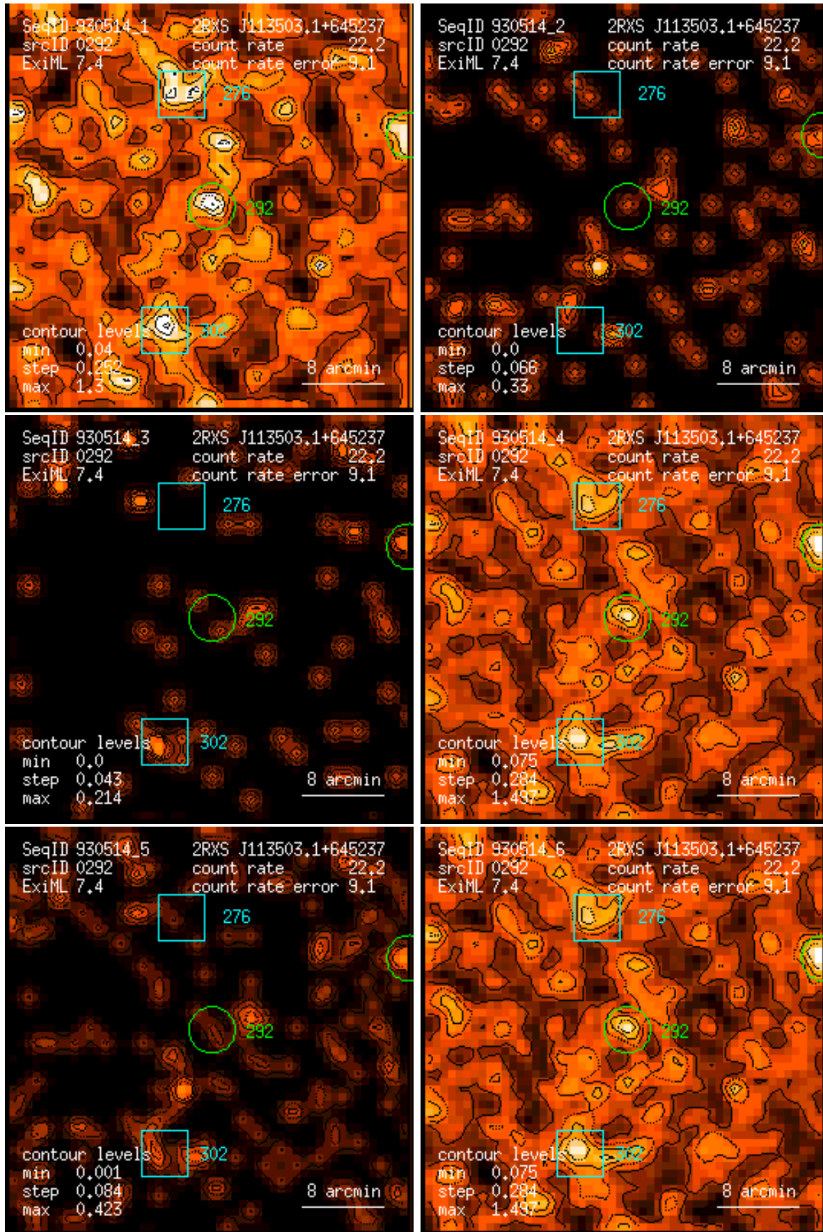
Figure 292: RASS 930514: detection 0292: band rate images, Gaussian filter: (1) PSPC channels 11 – 41, (2) 52 – 90, (3) 91 – 201, (4) 11 – 235, (5) 52 – 201, (6) 11 – 201. Broad band rates in counts/ks. Band rate contour levels in counts/ks/arcmin 2 .
